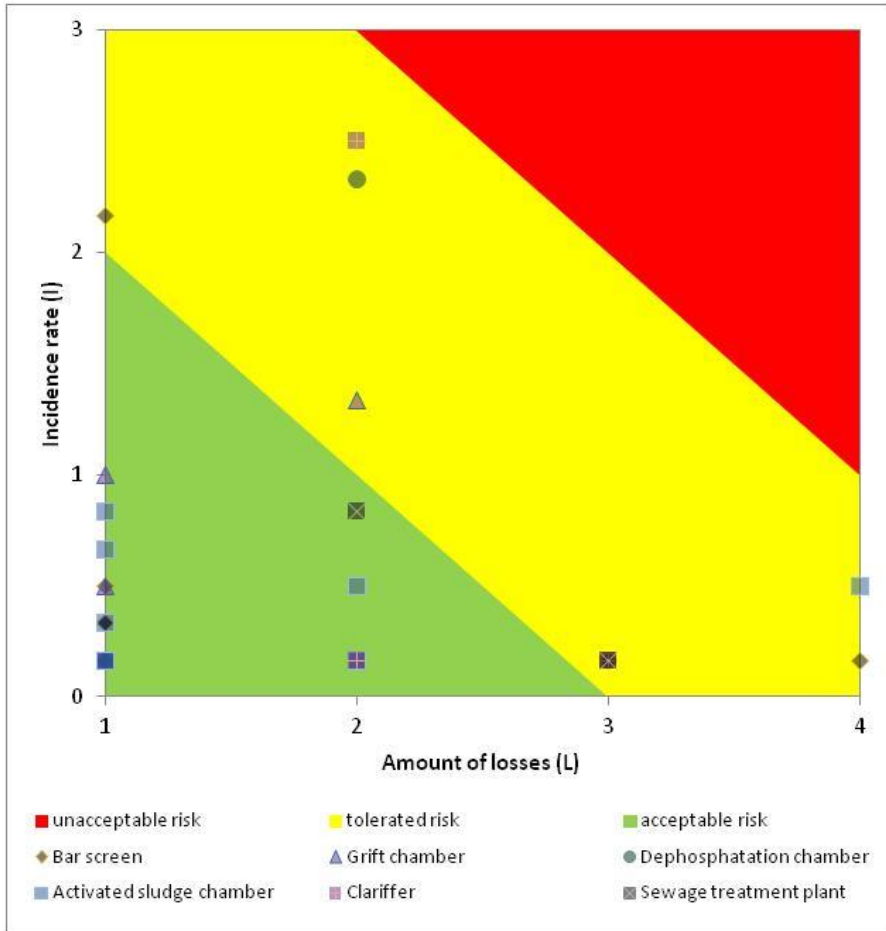
Fig. 4. A risk map taking into account its hierarchy with division into technological line devices
