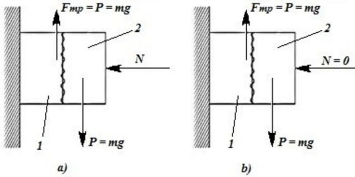
Fig. 2. Contacting friction surfaces
