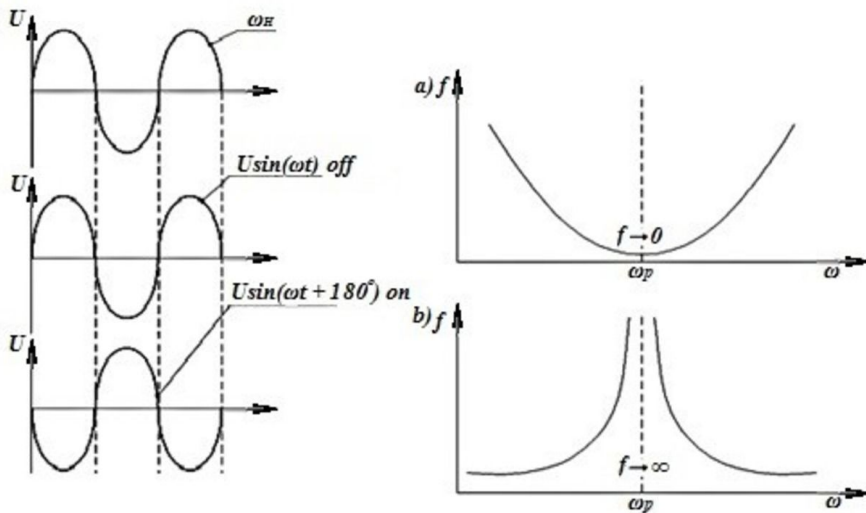
Fig. 5. Schedules of steering dynamic interaction on a frictional contact area.
