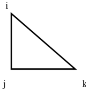
Fig. 1. The triangular finite element of the computational domain.
