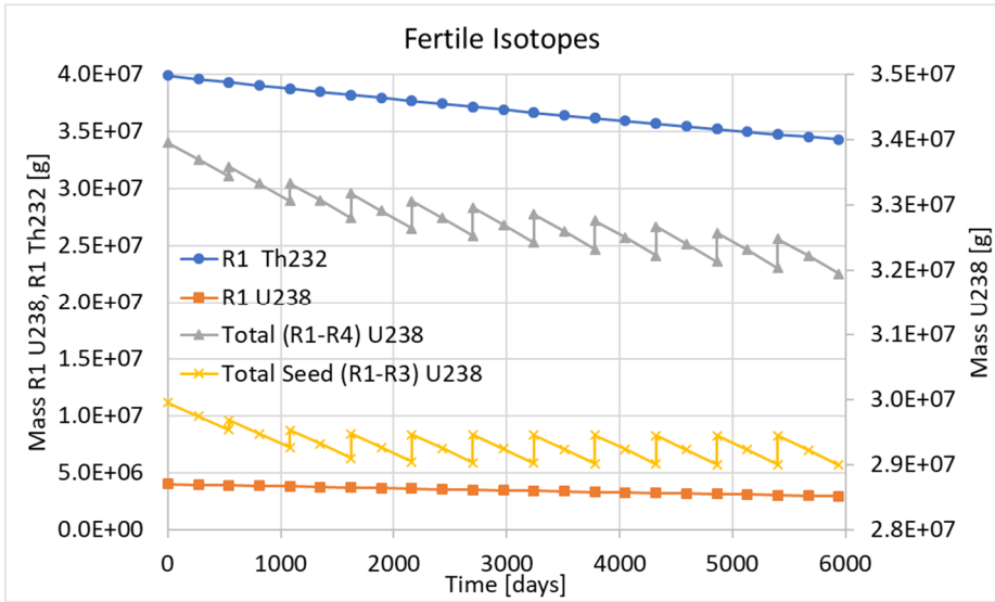
Fig. 3. Time evolution of fertile isotopes.
