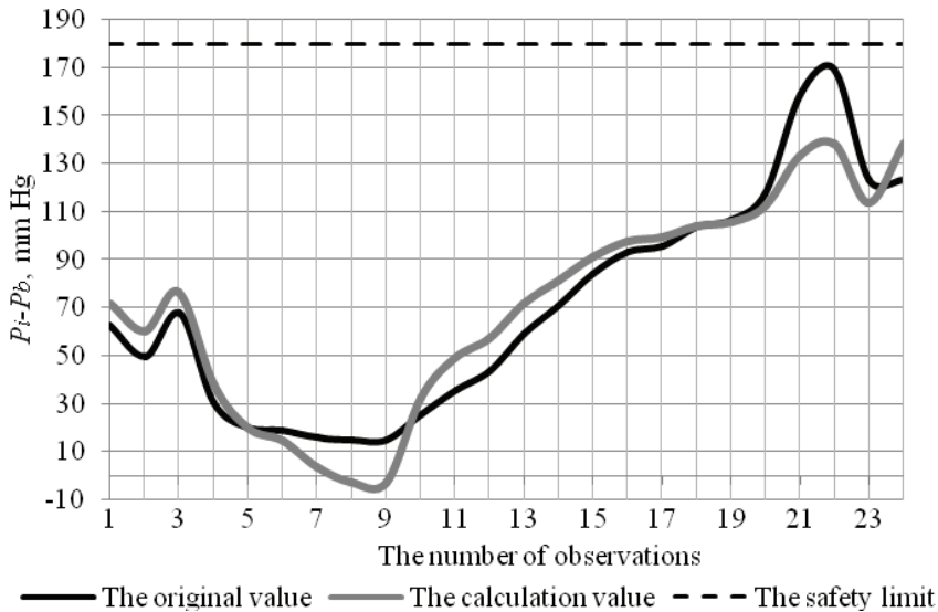
Fig. 2. Dynamics of changes in the pressure of the methane-air mixture of original and value calculation.
