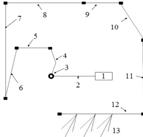
Fig. 1. Scheme of the underground pipeline 24 WSW: 1 - vacuum pump station; 2 - surface gas pipeline l = 50 m; 3 - borehole «1175» l = 915 m; 4 - degassing passage l = 30 m; 5 - air passage l = 70 m; 6 - air winze l = 40 m; 7 - conveyor incline l = 300 m; 8 - east main conveyor drift l = 495 m; 9 - west conveyor drift l = 150 m; 10 - roadway with separate air ventilation l = 150 m; 11 - west flank air passage #23 l = 900 m; 12 - 24 west air drift l = 900 m; 13 - boreholes.
