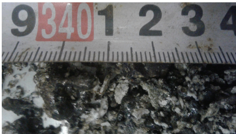
Fig. 3. Spalls of rock after the thermal reaming of the borehole by means of the angular plasmatron.
