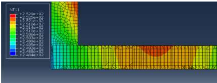
Fig. 14. The result of the calculation (the thermal conductivity brick is 0,6, 50.2 - steel).
