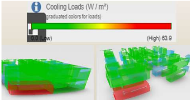
Fig. 11. Graph of cool load on the building.
