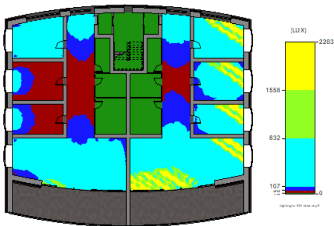
Fig. 12. Calculation output of lighting (blue – 50 lux, red – 107 lux).
