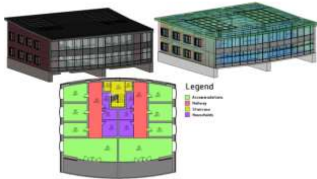
Fig. 1. 3D, analytical model and zoning plan.
