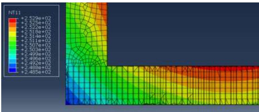
Fig. 15. The result of the calculation (the thermal conductivity brick is 0,6, 1,5 - basalt).
