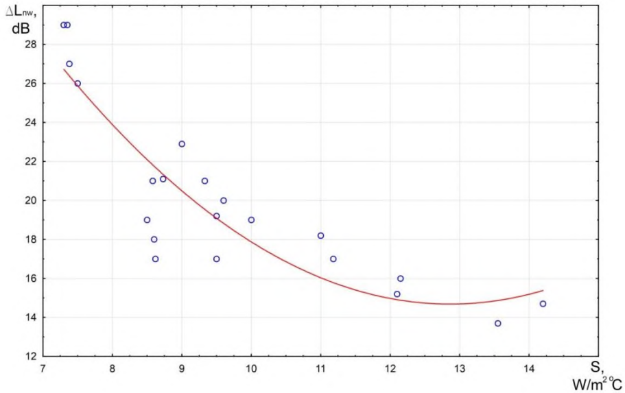
Fig. 2. The graph of correlation between heat absorption specific coefficient, S , and index of impact noise insulation improvement, \Delta L_{mw} for observed types of roll flooring materials.
