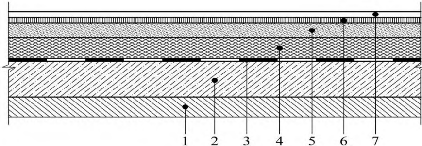
Fig. 1. The main construction layers of a floor construction: 1 - underlay; 2 - sub-floor; 3 - waterproofing; 4 - heat and sound insulation; 5 - topping; 6 - interlaminar layer; 7 – covering.
