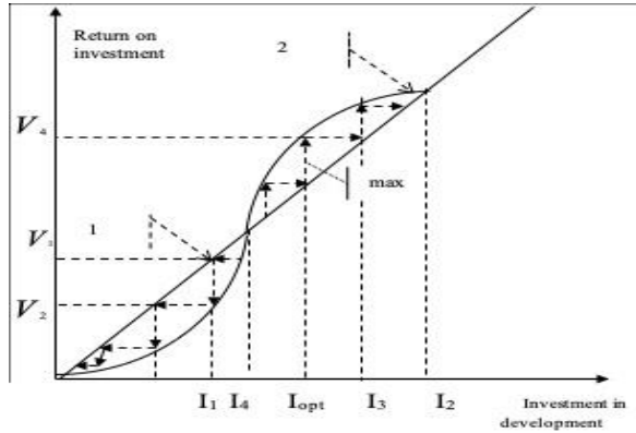
Fig. 2. S-model of possible development options of managed object
