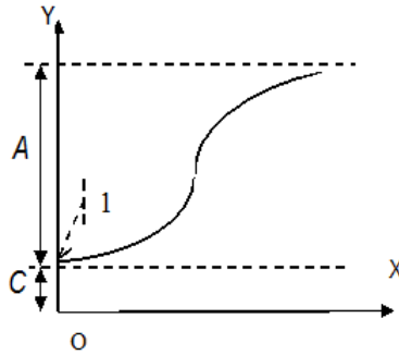
Fig. 1. S-curve corresponding to the Ferhulst equation
