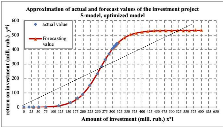
Fig. 3. Approximation of actual and forecast values of the investment project S-model, optimized model
