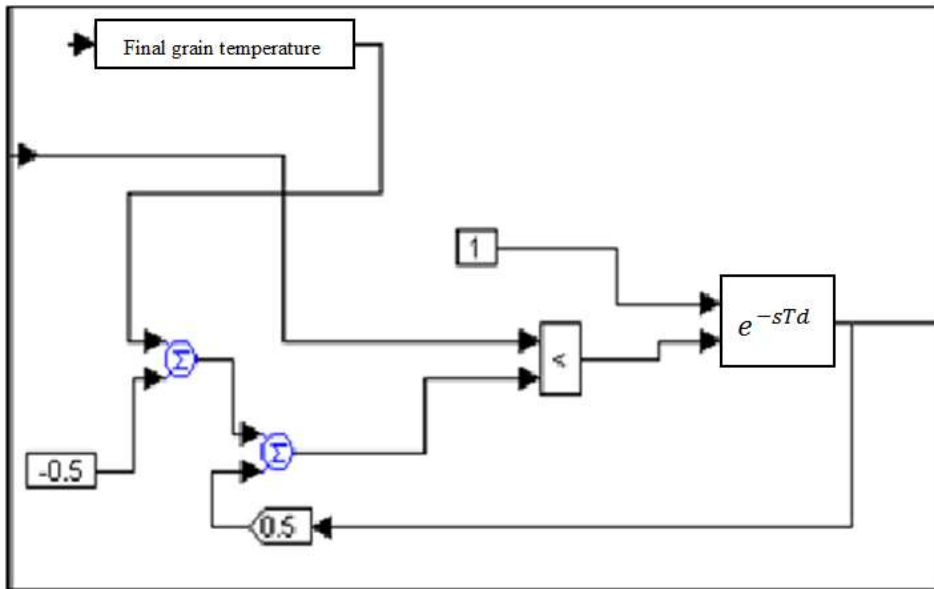
Fig. 2. Temperature control block.
