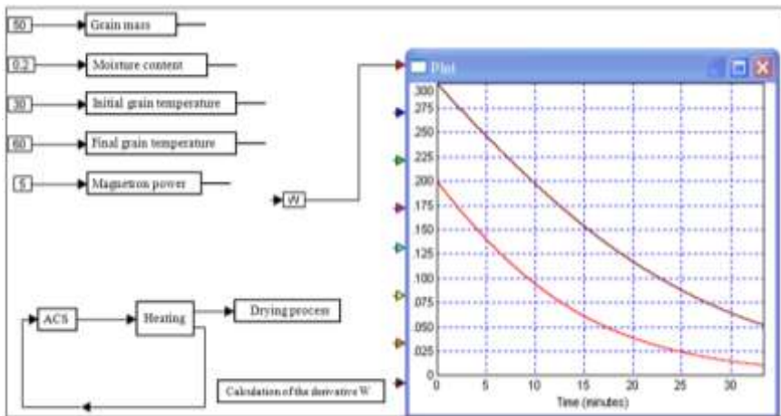
Fig. 5. The drying process at different values of the initial moisture content of the grain.
