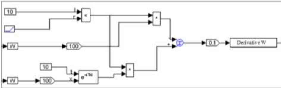
Fig. 7. The block “Calculation of the Derivative W ” in the expose form.
