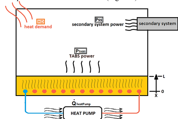
Fig. 3. Energy balance in a building, schematic interaction between heat demand, secondary system, and GEOTABS.
