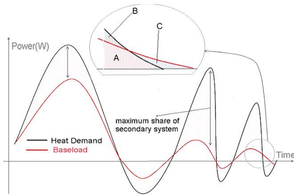
Fig. 1. Share of TABS and secondary system from heat demand
