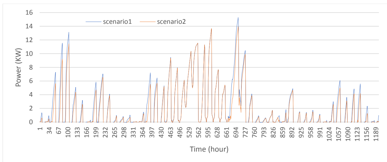
Figure 4. Share of the secondary system in case number 2 for both scenarios for 50 days starting from January 10th
