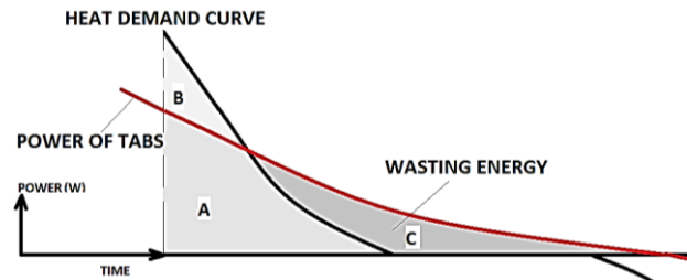
Fig. 2. An example of problematic moments in hybridGEOTABS. “A” is heat from surface of TABS, “B” is the heat of secondary system, and “C” is heat from TABS and secondary system in opposite sides at the same time, and thus called wasted energy
