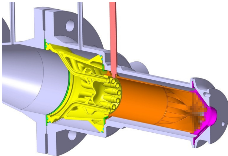
Fig. 1. Combustion chamber overview with integral combustor and fuel plenum (yellow), liner (orange), outlet (pink) and ignitor (red).
