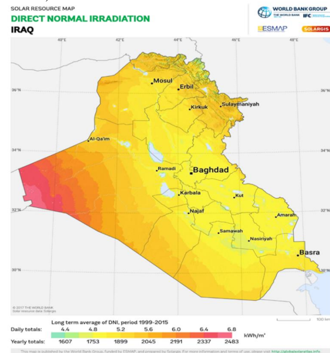
Fig.2. Iraq solar density
