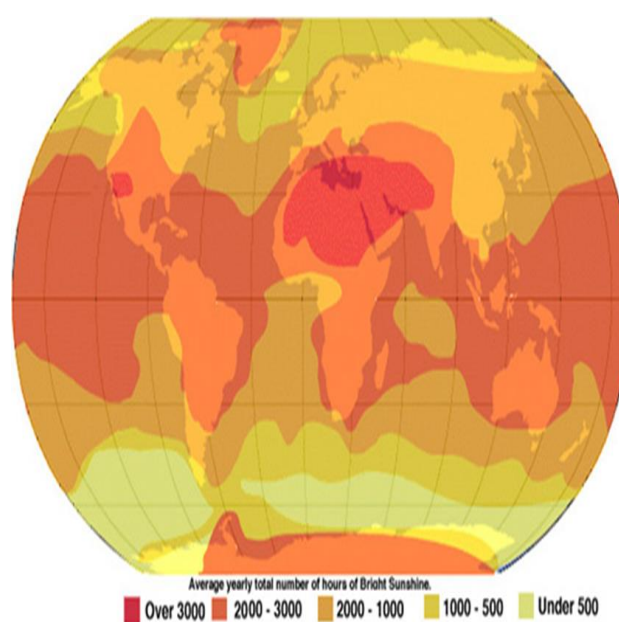
Fig. 3. Average yearly total numbers of hours of bright sunshine
