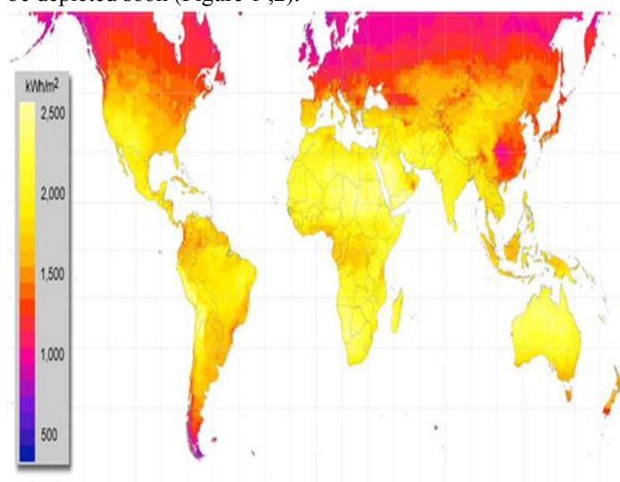
Fig.1. Iraq location at global irradiance (1850-2400 kwh/m 2 )
