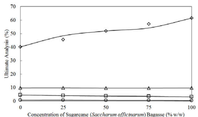
Fig. 2. Comparison of experimental values for ultimate analysis parameters – carbon (◇), hydrogen (□), nitrogen (△), and sulfur (○) versus calculated values (solid lines) based on linear additive rule.
