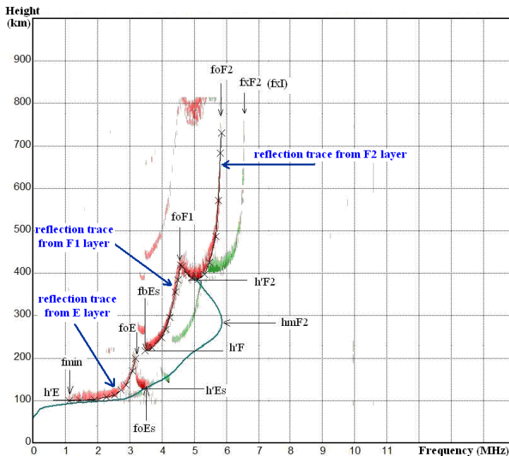
Fig. 3. Example of vertical sounding ionogram with main measurable parameters [6].
