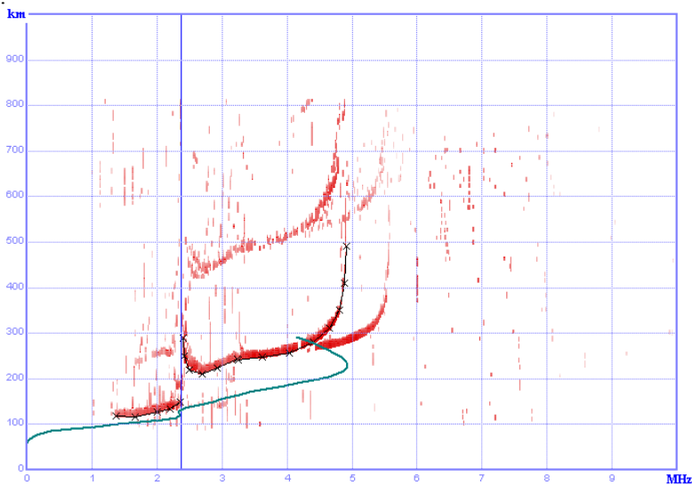
Fig. 6. An example of the extraction of the ionosphere parameter foE.
