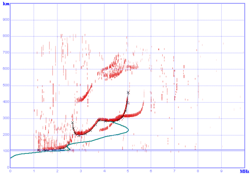
Fig. 9. An example of the extraction of the ionosphere parameter h'E.
