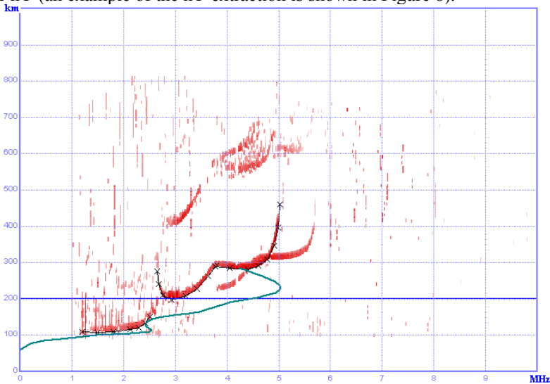
Fig. 8. An example of the extraction of the ionosphere parameter h'F.
