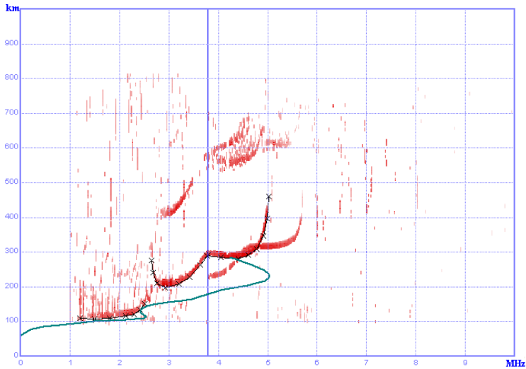
Fig. 5. An example of the extraction of the ionosphere parameter foF1.
