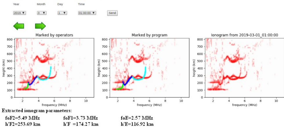
Fig. 10. An example of the extraction of the ionosphere parameter h'E.
