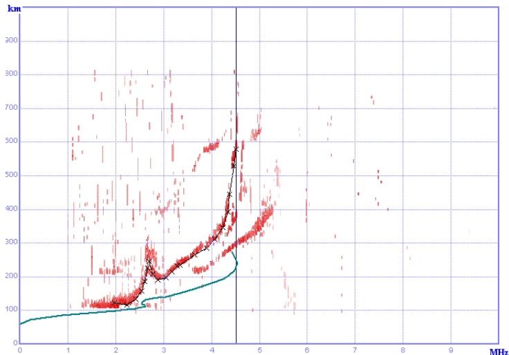
Fig. 4. An example of the extraction of the ionosphere parameter foF2.
