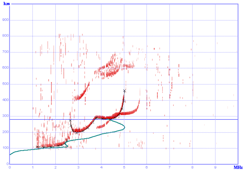
Fig. 7. An example of the extraction of the ionosphere parameter h'F2.
