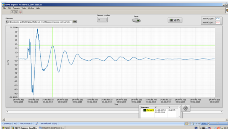
Fig. 7. Oscillogram of a single pulse recorded at the distance of 30 m from the radiator within the interval from 14:49:48.483 till 14:49:48.816 of local time.
