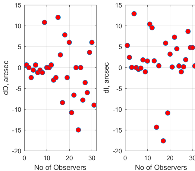
Figure 2. Errors of absolute values of declination D and inclination I obtained by 31 observers during the intercomparison of magnetometers at the IAGA Workshop in Hyderabad in 2014.
