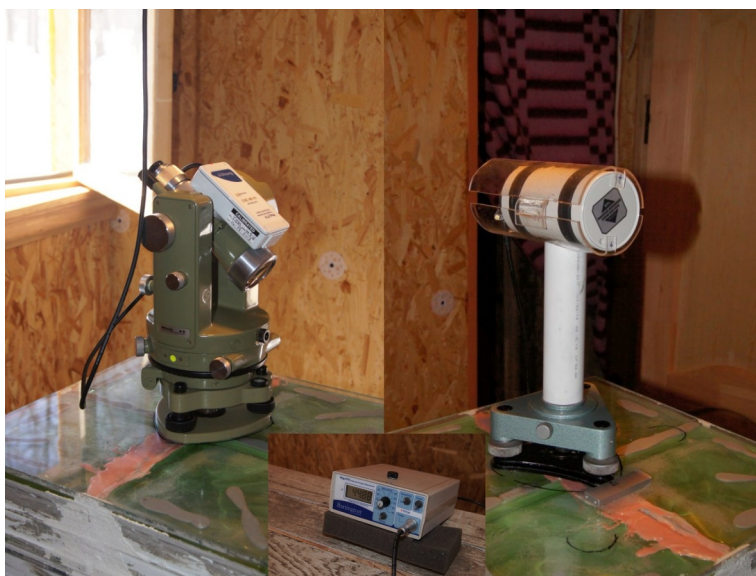
Figure 1. Absolute magnetometers: DIflux Mag-01H (left) with electronics (in frame) and Overhauser scalar magnetometer POS-1 (right) at Geophysical Observatory Paratunka (PET).
