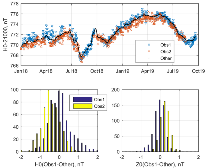
Figure 3. Personal differences of observers according to the results of absolute measurements at the Observatory Paratunka (PET) in 2018-2019. Upper panel — the baseline values of H0 for two observers and the average value for the other three observers (approximation for each hour). Bottom panel: on the left — the distribution of deviations of individual values of H0 of two observers from the system of other observers, on the right—the same for the component Z0.
