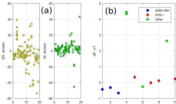
Figure 4. The results of intercomparison of absolute magnetometers. (a) deviations of absolute values of \mathbf{D} and \mathbf{I} of compared DIFluxes from reference DIFlux, Observatory Kakioka, Japan (2004). (b) deviations of total field intensity values \mathbf{F} of compared scalar magnetometers from reference device obtained during intercomparison at Observatory Arti, 2017. Numbers at abscissa are presented conditional number of magnetometer.
