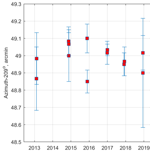
Figure 5. The results of astronomical observations of remote target at Observatory Paratunka. Squares ■ define the mean values of the azimuth, vertical bars are standard deviations for results of the daily measurements.
