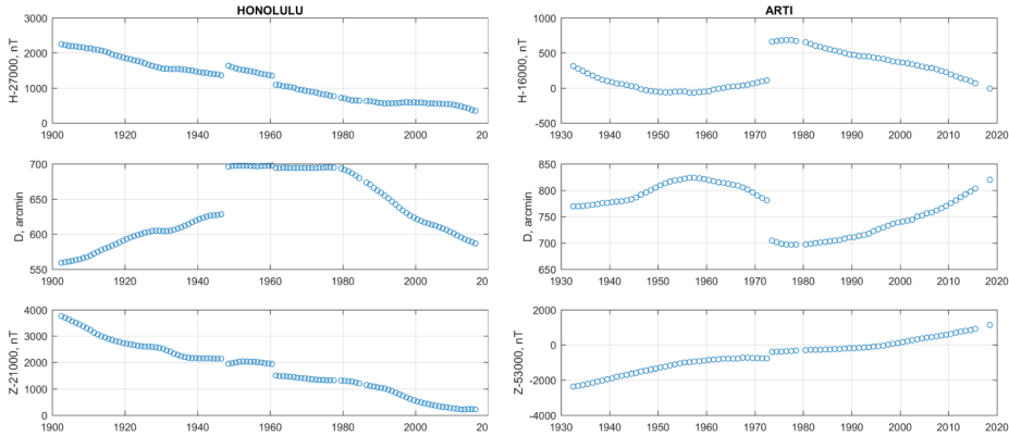
Figure 6. Examples of jumps in yearmean data records at magnetic observatories Honolulu and Arti due to moving to new locations.
