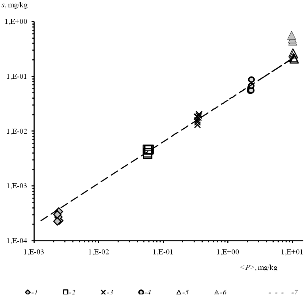
Figure 1. The relationship between the time average concentrations \langle P \rangle and the sample standards s for the hydrochemical parameters measured in the Ezcurra Inlet at depths of 1, 5, 10, 15, 20, 30, 40, 50, 60, and 70 m (bottom) for 0.5-2.3 months. 1-7 – nitrite, phosphate, nitrate, silicate, dissolved oxygen, dissolved oxygen only at depths of 50, 60, and 70 m, and power law regression, respectively (see initial data in [8]). Phosphates, nitrates, and silicates varying statistically insignificantly are not shown.
