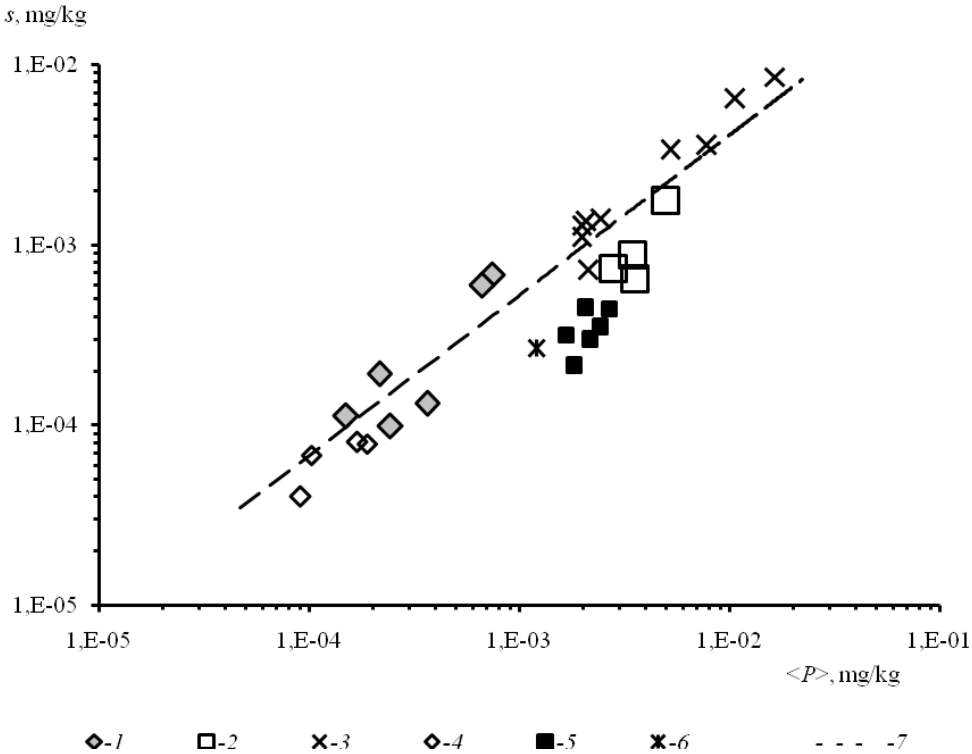
Figure 2. The relationship between the time average concentrations \langle P \rangle and the sample standards s for the complex of hydrochemical parameters at the daily station in the Sargasso Sea at depths of 0, 15, 25, 50, 75, 100, 125, 150, 200, 300 m. 1-3 – nitrite, phosphate, nitrate with significant daily fluctuations, respectively; 4-6 – nitrite (15, 25, 50, 300 m), phosphate (15, 25, 50, 75, 100, 125 m), nitrate (50 m) with insignificant at 95% level daily fluctuations, respectively; 7 – power regression (see initial data in [9]).
