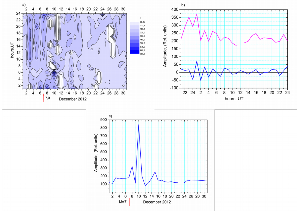
Fig 2. a) Atmospheric amplitude variations in December 2012; b) atmospheric amplitude variations in December 6UT; c) amplitude variations December 15.
