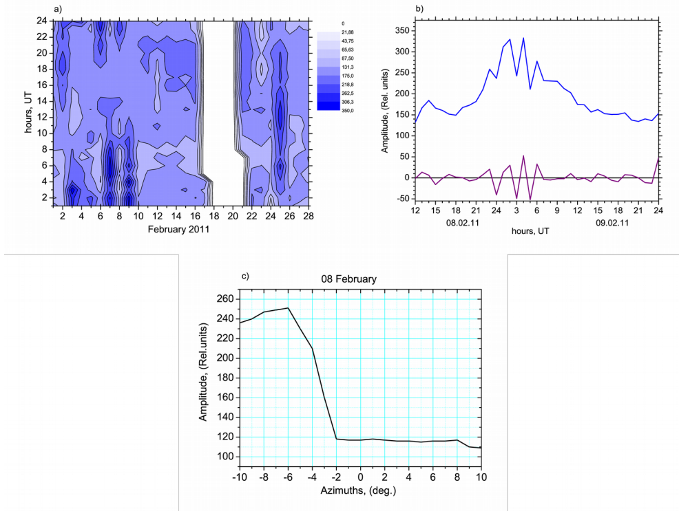
Fig 1. (a) Variations of the amplitude of lightning discharges in February 2011 at all hours of the day. Variations of amplitude are shown by color intensity, white color - no data (February 17-22); (b) atmospheric amplitude variations on February 8 and 9; (c) azimuthal distribution of atmospheric amplitudes from directions on earthquake.
