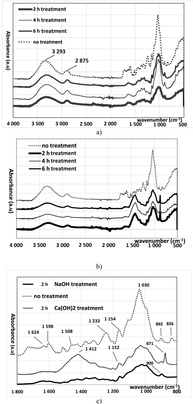
Fig. 2 FTIR spectra of untreated and treated bagasse fibers in the region between 500\text{ cm}^{-1} to 4\,000 in a) NaOH and b) \text{Ca(OH)}_2 and c) in the region between 800\text{ cm}^{-1} to 1\,800\text{ cm}^{-1} for 2 h treatment in NaOH and \text{Ca(OH)}_2 .
