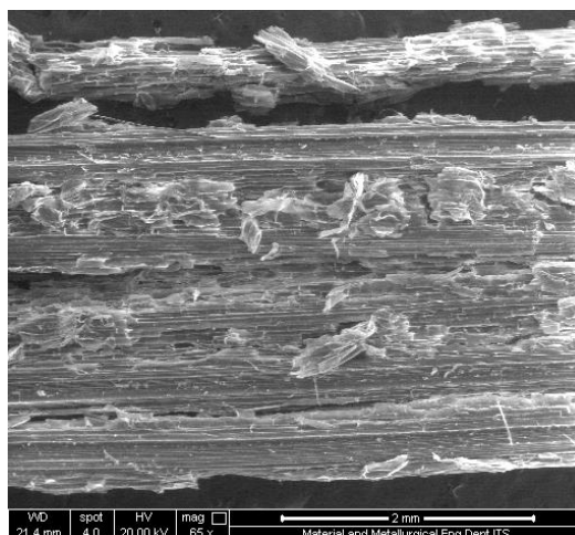
Fig. 4. SEM micrographs of longitudinal view of untreated sugar cane fibers.
