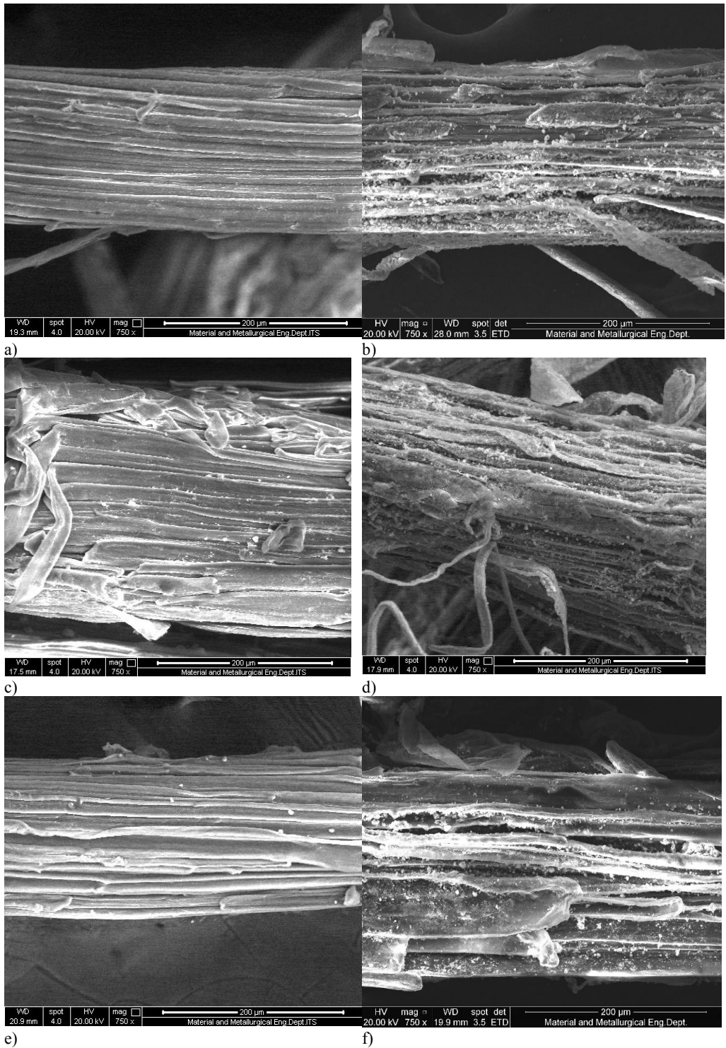
Fig. 5. SEM micrographs of bagasse fibers after treated using NaOH for a) 2 h, c) 4 h, and e) 6 h and using Ca(OH) 2 for b) 2 h, d) 4 h, and f) 6 h.
