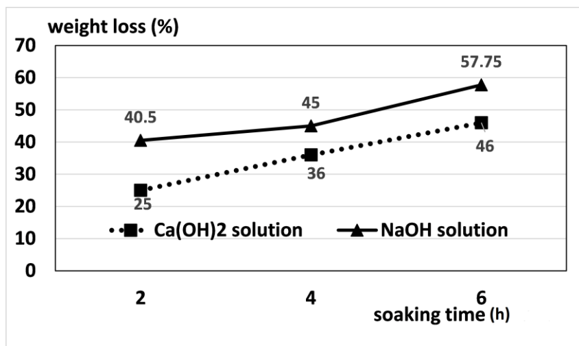
Fig. 1. Weight loss of bagasse fibers after treatment.
