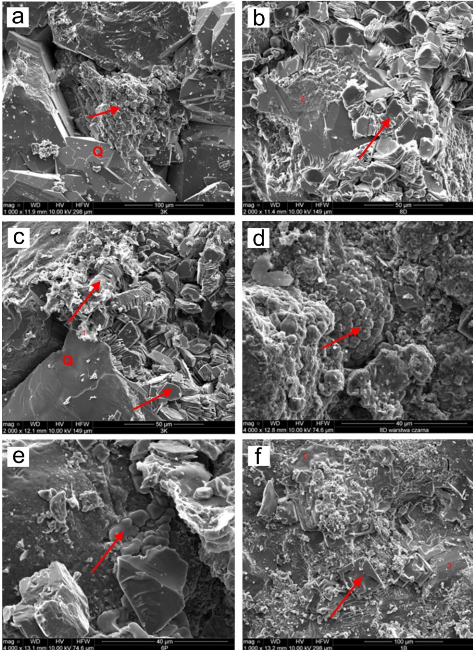
Fig. 3. Microstructures of sandstones samples found in the Lower Jurassic boreholes cores: a – regenerative quartz cement (Koło IG-4: 2732.5 m b.g.l.); b – kaolinite cement (Damaśławek 22: 3391.3 m b.g.l.); c – kaolinite cement (Koło IG-3: 3079.4 m b.g.l.); d – ferruginous-clay cement (Damaśławek 22: 3391.3 m b.g.l.); e – halite efflorescences in the form of amorphous encrustations (Poddębice PIG-2: 3364.5 m b.g.l.); f – halite efflorescences in the form of crystals with a regular habit (Banachów IG-1: 3344.5 m b.g.l.).
