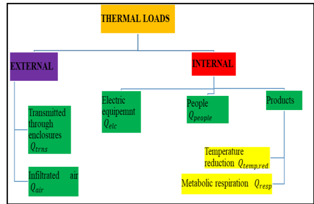
Fig. 4. Classification of thermal loads existing in cold chambers [9].
