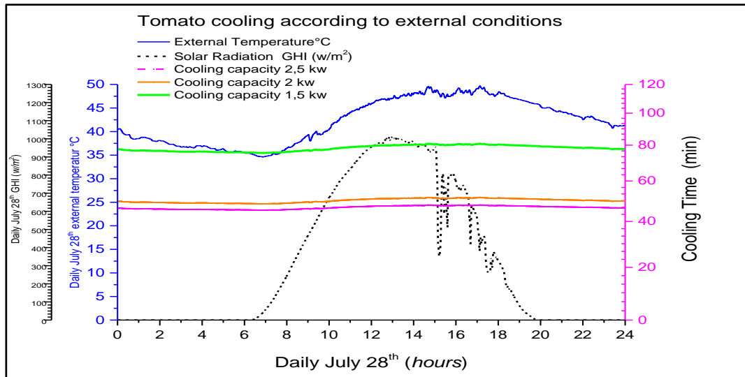
Fig. 5. Tomato cooling time by external condition.
