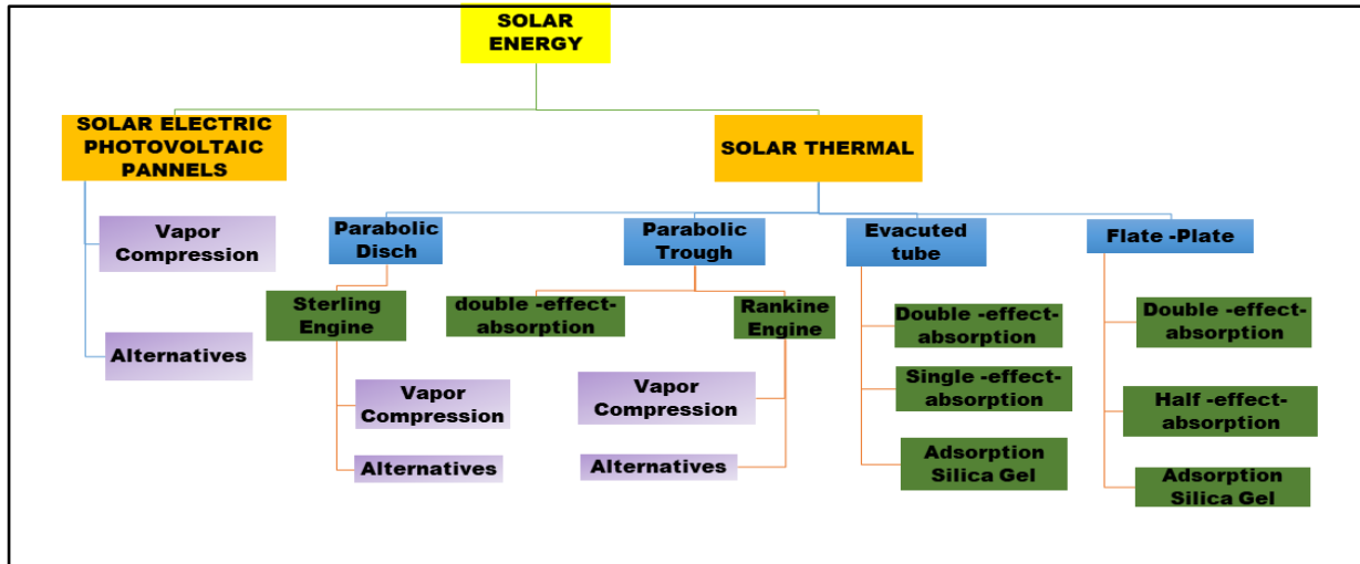
Fig.1. Alternative routes from solar energy into cooling effect using thermodynamic cycles [1]
