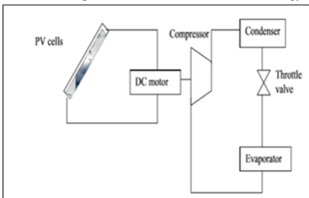
Fig. 2. Schematic of a PV-driven vapor Compression chiller [6].
