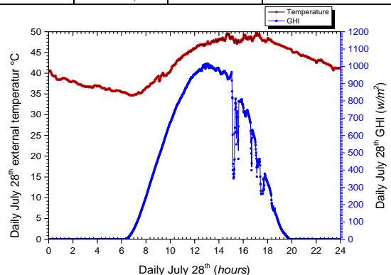
Fig.3. Summary GHI and External Temperature of Daily July 28th [8].
