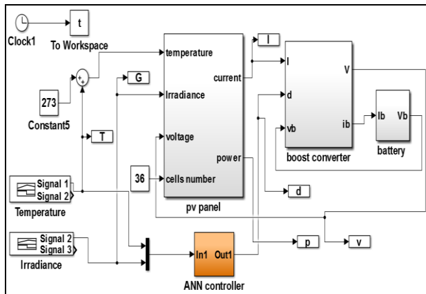
Fig.7. Matlab/Simulink Block diagram of the PV system with the proposed ANN controller
