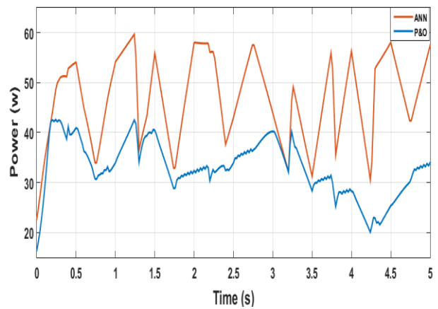
Fig. 13. PV output power case of random variation of irradiance and temperature.
