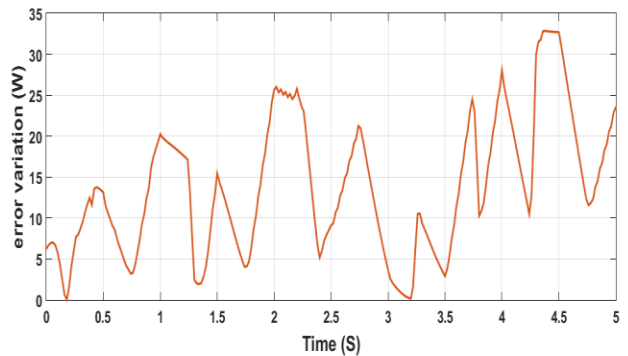
Fig. 14. Power error variation case of random variation of irradiance and temperature
