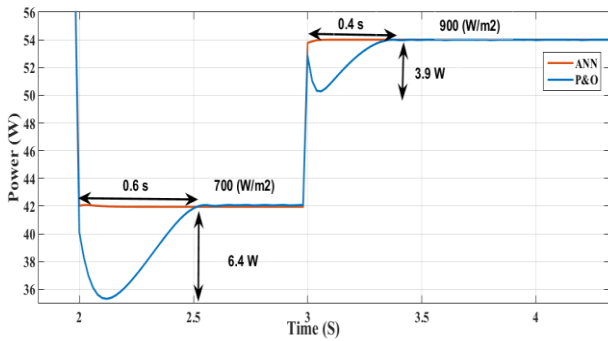
Fig. 10. Zoom on overshoot case of irradiance increase and decrease
