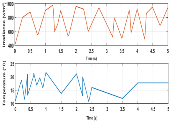
Fig. 11. Random variation of irradiance and temperature.
