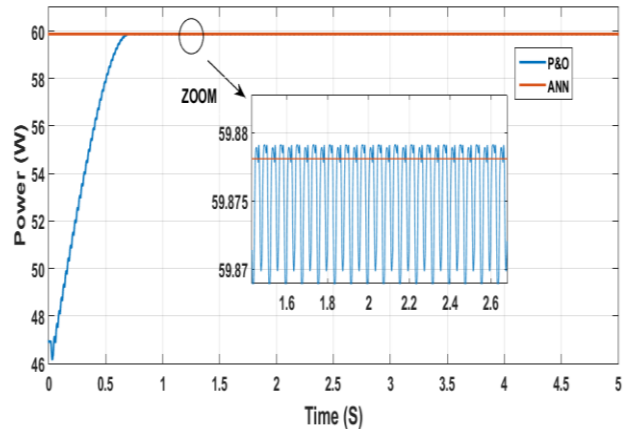
Fig. 8. MPPT simulation of the P&O and ANN methods under STC.
