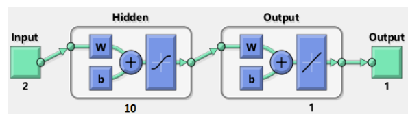
Fig. 5. The proposed neural network architecture in Matlab.
