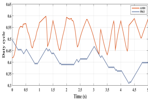
Fig. 12. Duty cycle case of random variation of irradiance and temperature
