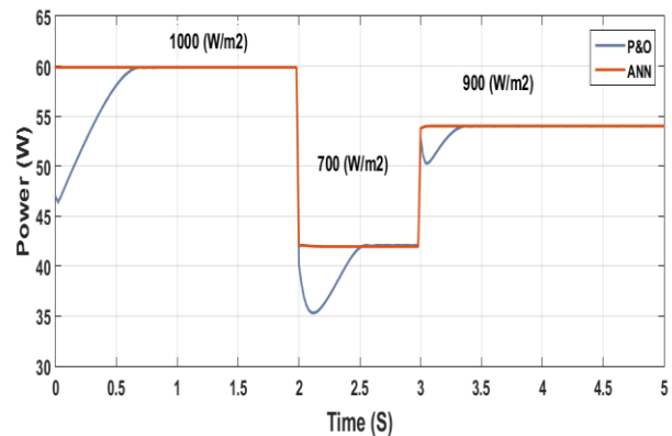
Fig. 9. PV output power case of irradiance change
