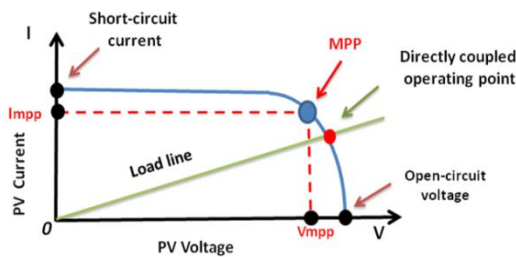
Fig. 2. I-V characteristics of PV system
