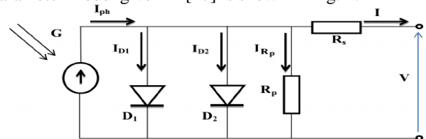
Fig. 1. Two diodes cell model.
