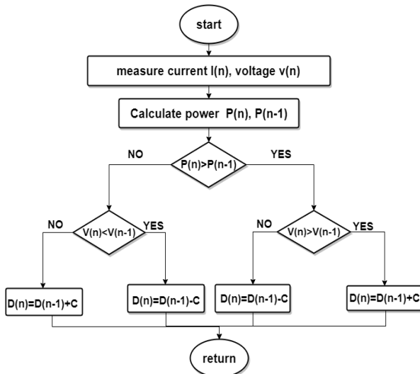
Fig. 3. Flowchart of the P&O algorithm
