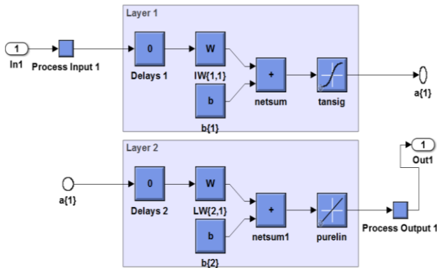
Fig. 6. Unmasked ANN controller subsystem
