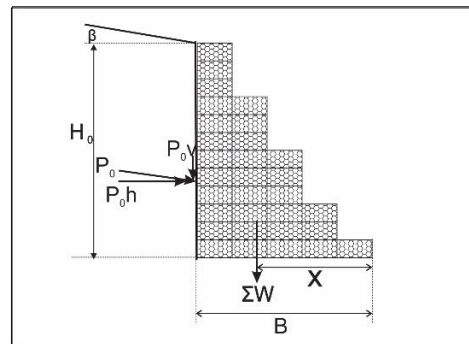
Fig.3a. illustration for overturning stability (initial)
