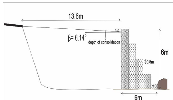
Fig. 6b. cross section (after sliding)
