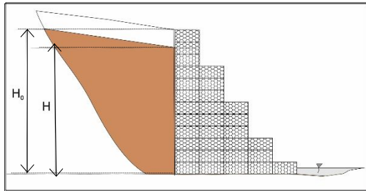
Fig. 1. back fill height at present (H) and initial (H 0 ) condition
