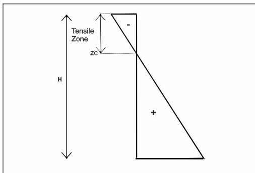
Fig. 2. active lateral pressure diagram
