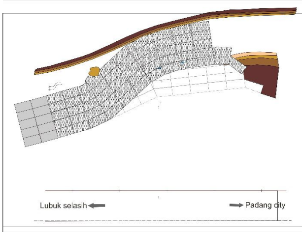
Fig.5b. Plan view of the gabion retaining wall after sliding
