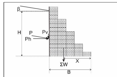
Fig.3b. illustration for overturning stability (present)
