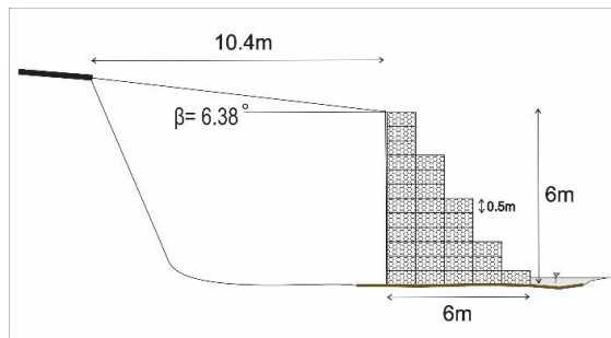
Fig.6a. cross section (before sliding)
