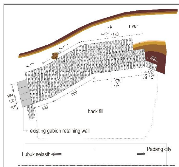
Fig.5a. Plan view of the gabion retaining wall before sliding
