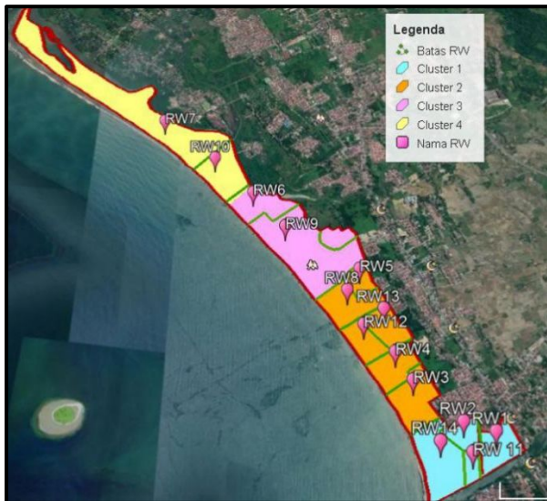
Fig. 4. Clusters position
