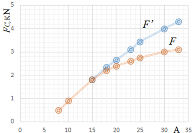
Fig. 4. Power force on the secondary element for two structures
