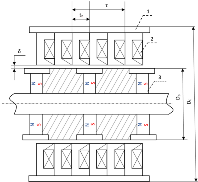
Fig. 1. CLVD in longitudinal section
