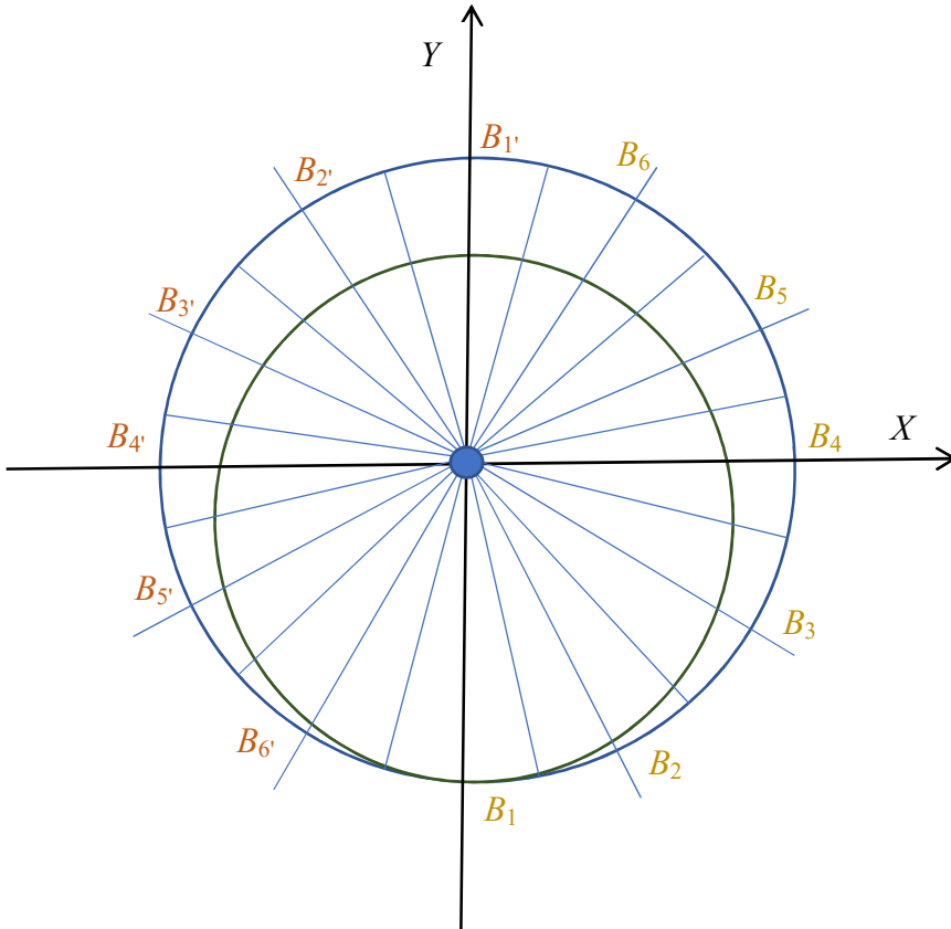
Fig. 2. Breakdown of the diameter of the magnetic system of the CLVD into sectors
