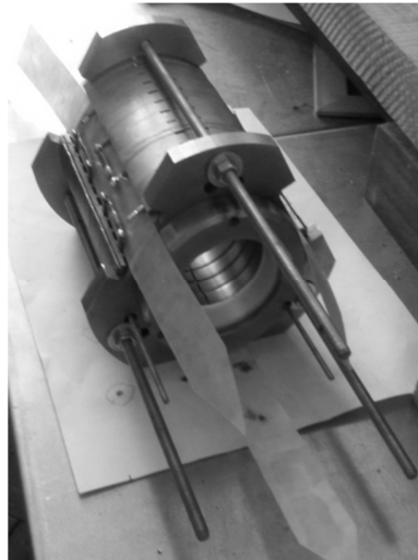
Fig. 3. Inductor with three symmetrical slots
