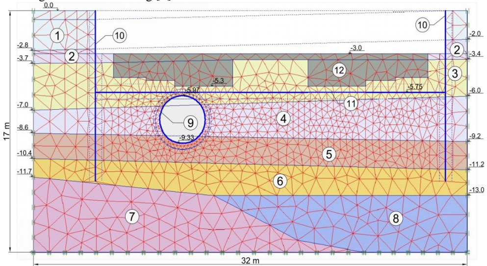
Fig. 9. The accepted analytic model: 1 – fill-up ground: soft sandy loam; 2 – silty sand; 3 – very soft loam; 4 – banded sluffing soft loam; 5 – banded sluffing soft loam; 6 – very soft laminated loam; 7 – soft sandy loam; 8 – semi-solid soft loam; 9 – sewer lining; 10 – grooved bracing; 11 – pipe, Ø530 mm; 12 – existing foundation of the church.
