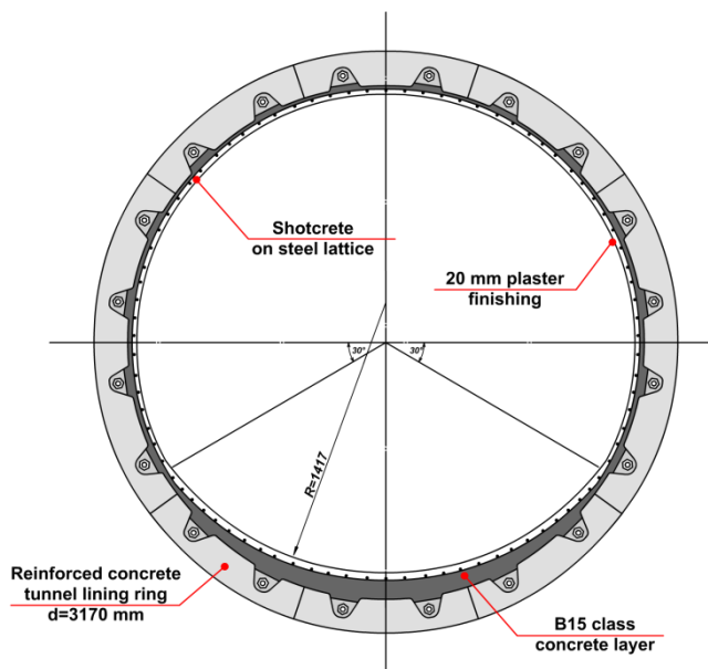
Fig. 3. TKK23 sewer tunnel lining cross-section affected by the re-erection of the object of cultural heritage
