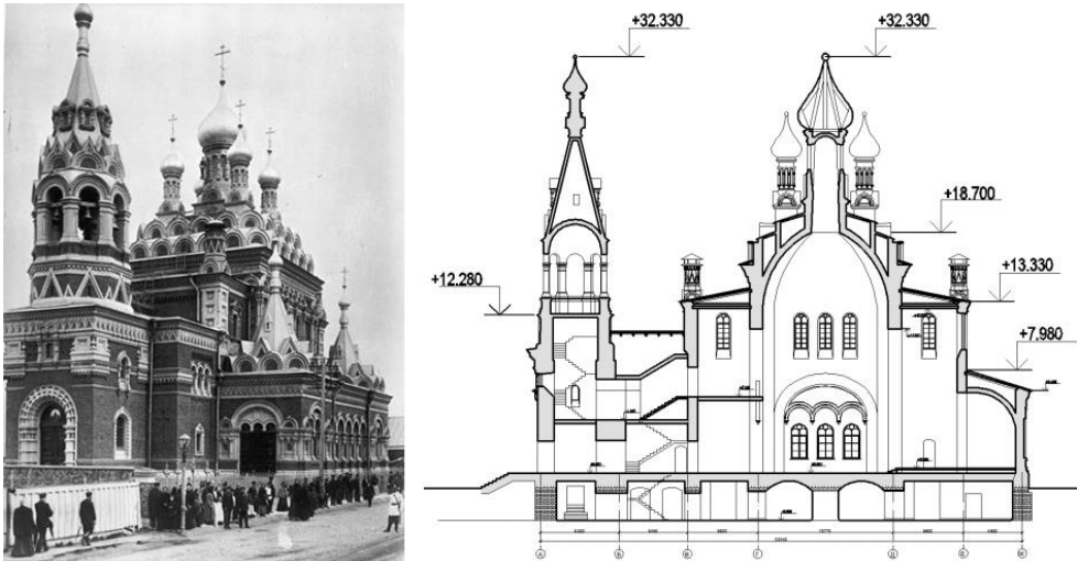
Fig. 2. The general view and the cross-section of the Church of Our Lady Joy of All Who Sorrow before demolition
