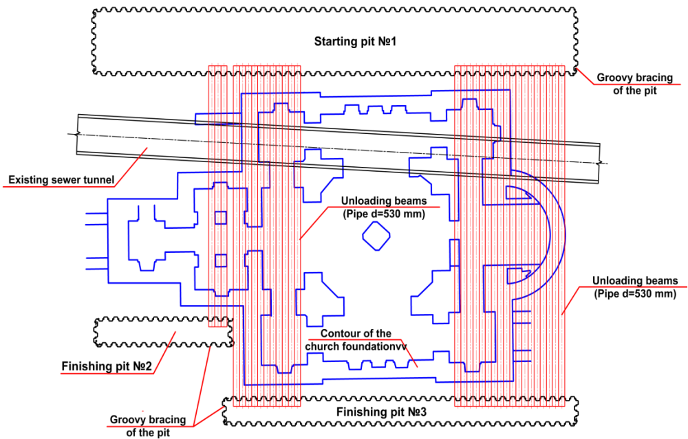
Fig. 4. Layout of reinforcement girders under the church foundation
