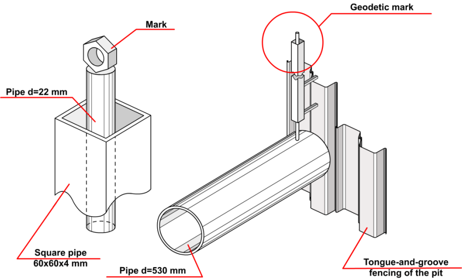
Fig. 5. A geodetic mark scheme
