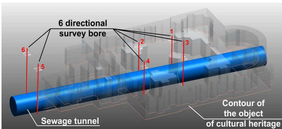
Fig. 8. Layout of survey bore sensors
