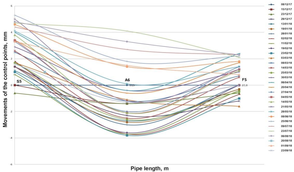
Fig. 6. A diagram of movements of geodetic marks control points
