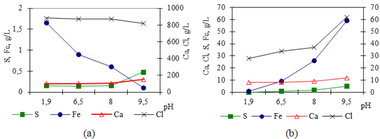
Fig. 3. Effect of pH on concentration of elements in solid (a) and liquid (b) phase.
