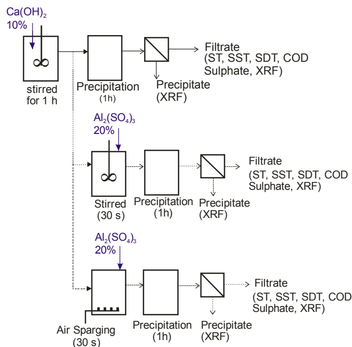
Fig. 2. The block diagram of studied wastewater treatment process.
