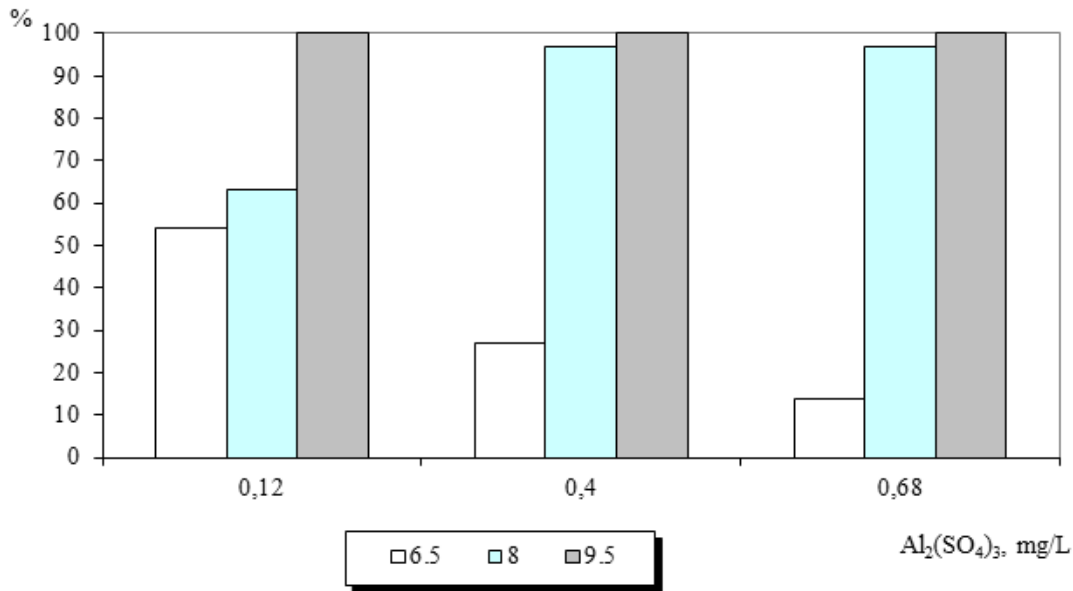
Fig. 3. Effect Al 2 (SO 4 ) 3 dosage on removal turbidity at different pH.
