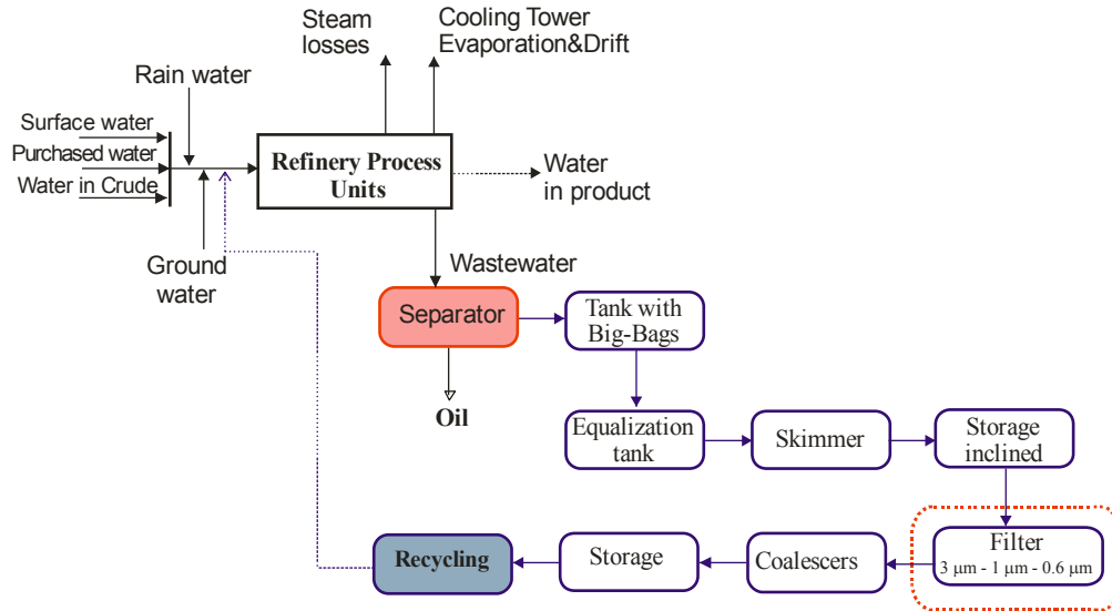
Fig. 1. The block diagram of the wastewater treatment process produced in the Centre Treatment Oil ROM, Hassi Messaoud, Algeria.
