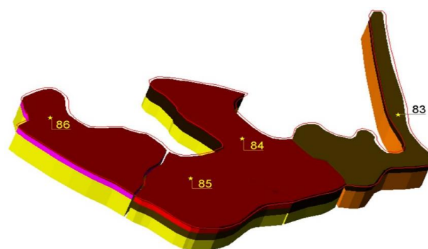
Fig. 3. The 3D-model of oil pollution of the site 2.7. 2598.
