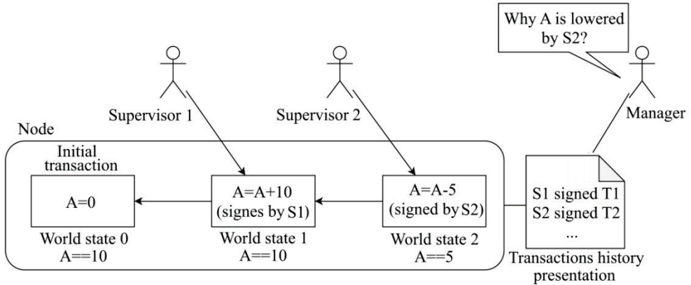
Fig. 2. Blockchain write error correction.
