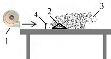
Fig. 1. Sketch of the laboratory setup: 1 – fan; 2 – model of the coal pile; 3 – contamination zone; 4 – barrier.
