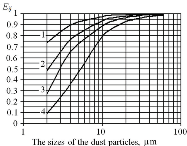
Fig. 3. Dependences of the capture coefficient E_{ij} of particles with drops from the size of particles at a relative speed of their movement of 5 m/s: 1, 2, 3, 4- for the diameters of drops 10; 40; 100 and 600 microns, respectively.
