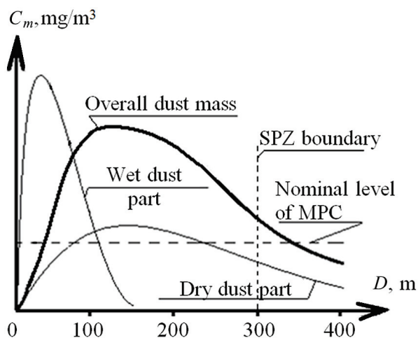
Fig. 4. The qualitative nature of the change in the surface concentration C_m of the total dust mass released into the atmosphere at the sites of dust formation, and its components - not wet (dry) and wetted parts of dust formed in the case of dust hydro irrigation in the direction of wind.
