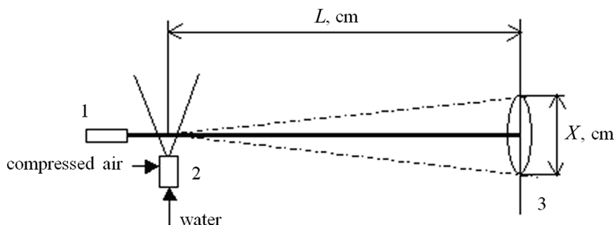
Fig. 1. Scheme for determining the droplets size of spray liquid: 1– laser emitter; 2 – water irrigator (sprayer); 3 – screen.
