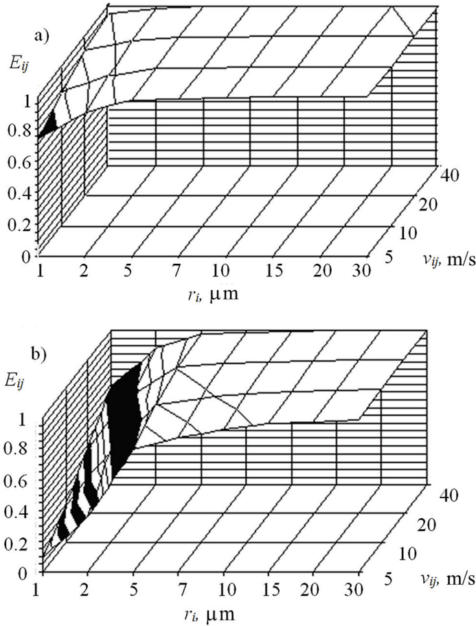
Fig. 2. Dependence of the capture efficiency of particles with different radius r_i by drops at different relative speed of their motion v_{ij} : a, b – respectively for drops of radius R_j = 5 and 300 \mu\text{m} (the diameter of droplets 2R_j is respectively 10 and 600 \mu\text{m} ).
