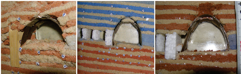
Fig. 3. General view of the roadways and protective constructions in the models.
