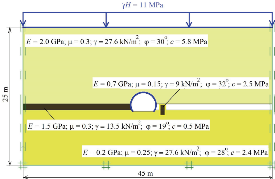
Fig. 4. General view of the numerical model at the stage of its construction ( E – elastic moduli; \mu – the Poisson coefficient; \gamma – volume weight; \phi – angle of internal friction; c – adhesion; H – depth of work).
