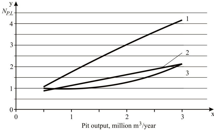
Fig. 3. The dependence of the pipelines number for placing sand in the internal sludge pond from the production capacity of the quarry: 1, 2, 3 – pipeline diameter ( D_T ) – 200, 400, 600 mm, accordingly.
