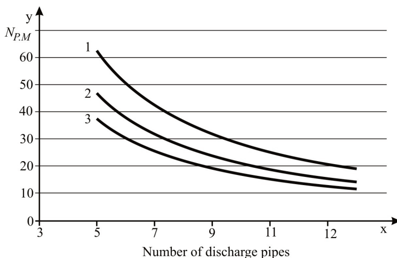
Fig. 4. The dependence of the pipeline movement number in sludge pond on the discharge pipes number taking into account the distance between them: 1, 2, 3 – distance between discharge pipes – 6, 8, 10 m, accordingly.
