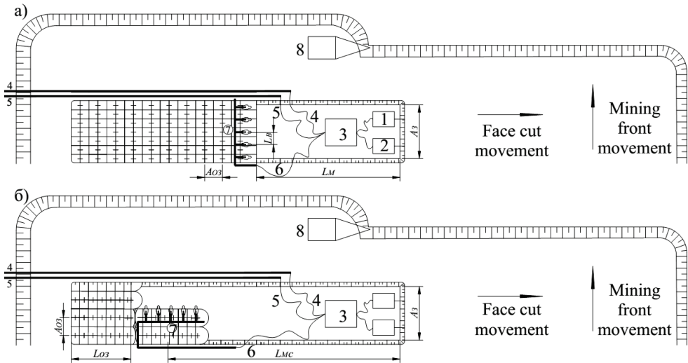
Fig. 6. The scheme for determining the sludge pond parameters in pit excavation: a) transverse; b) longitudinal; 1, 2, 3 – are the dredges and the floating processing plant as part of a hydromechanized mining complex; 4, 5, 6 – are the pipelines with heavy minerals, clay and sand rocks, respectively; 7 – is the sludge pond pipe with discharge pipes; 8 – is the shovel excavator.
