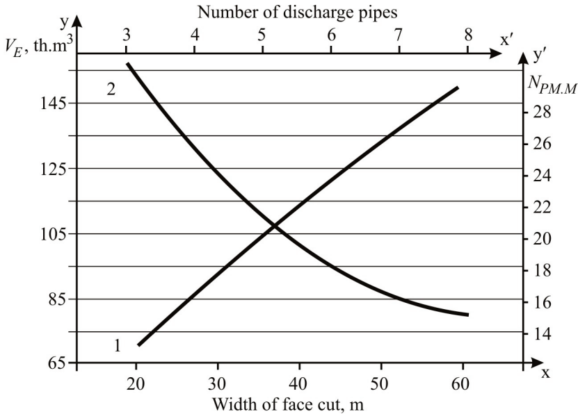
Fig. 7. The influence of the face cut width on the excavation volume and the number of pipeline with discharge pipes movements at the transverse scheme of sludge pond formation: 1 – excavation volume; 2 – number of pipeline.
