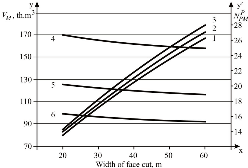
Fig. 8. The influence of the face cut width on average volume of excavation and the number of sludge pond pipeline movements taking into account the number of discharge pipes: 1, 2, 3 – volume of excavation at the number of discharge pipes – 6, 8, 10, accordingly; 4, 5, 6 – the number of discharge pipes movements in sludge pond at its number – 6, 8, 10, accordingly.
