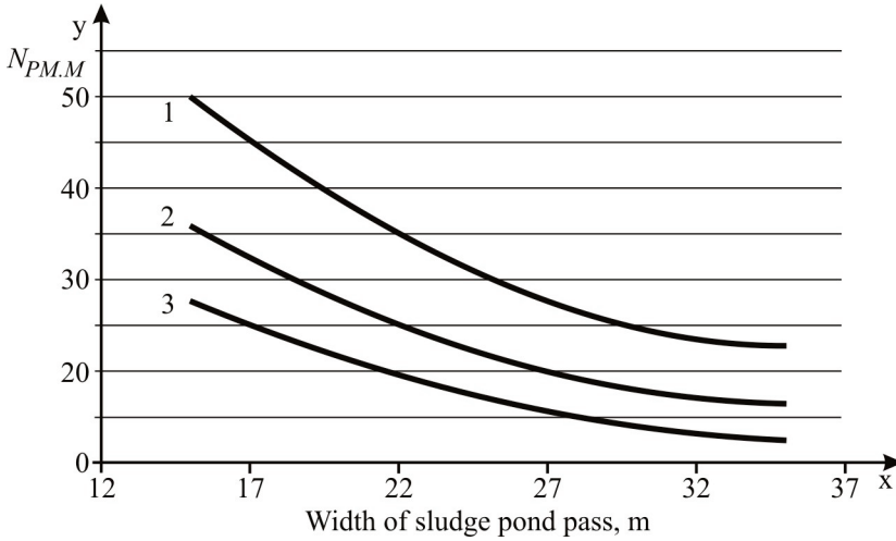
Fig. 5. The influence of the sludge pond pass width on the number of pipeline movements with the discharge pipes per month: 1, 2, 3 – distance between discharge pipes – 6, 8, 10 m, accordingly.
