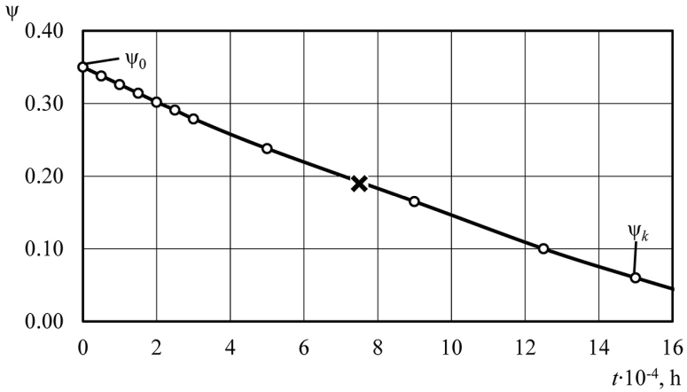
Fig. 4. Time dependence of energy absorption coefficient; \psi_0 and \psi_k are initial and final values of energy dissipation factor, \times – lower limit of the vibration isolator service life.
