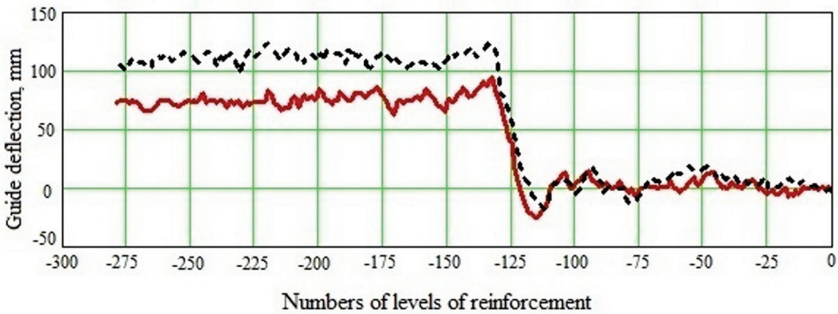
Fig. 4. Profiles of guides of an ore shaft in a zone of rock displacement of an ore-hoisting shaft in a lateral plane of guides.
