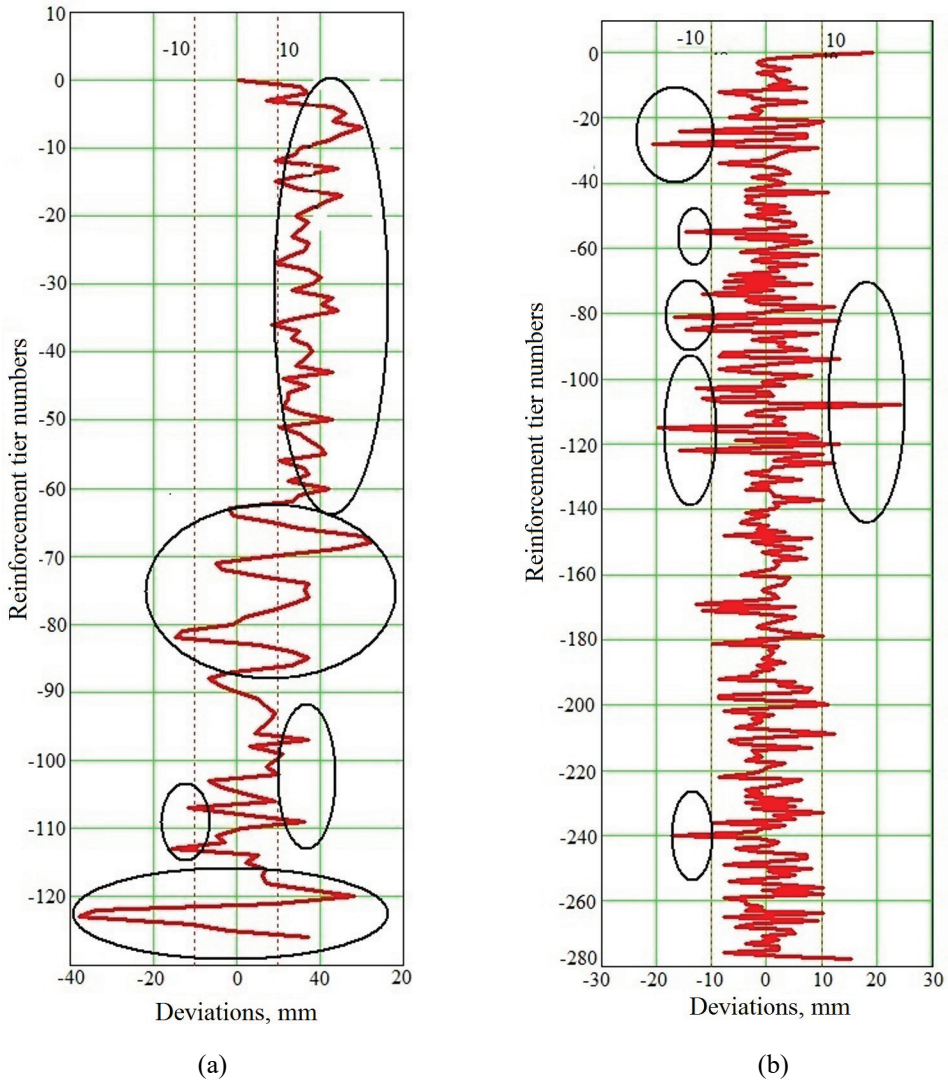
Fig. 9. Geometric parameters of guide profiles: deflections from the vertical on adjacent levels in a frontal plane of a coal shaft (a); ore shaft (b).
