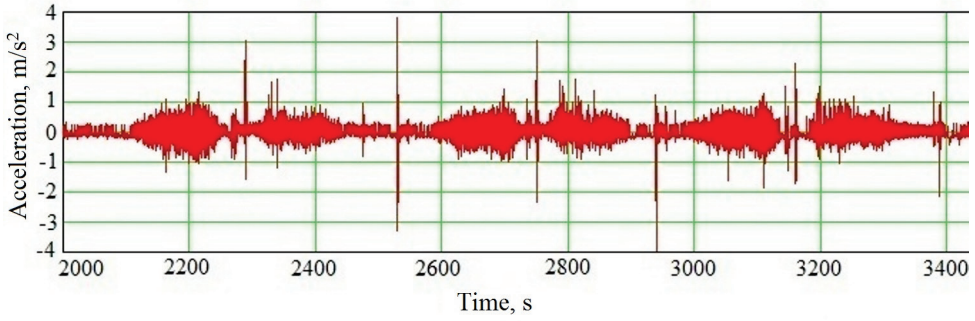
Fig. 11. Horizontal accelerations of vessel guides in frontal planes of reinforcement.
