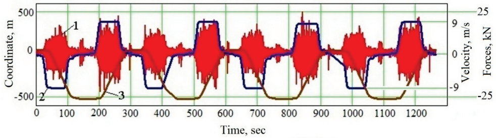
Fig. 13. Summary diagram of skip parameters: contact forces, velocities and coordinates in a shaft: 1 – forces, kN; 2 – velocity, m/s; 3 – coordinate in a shaft, m.
