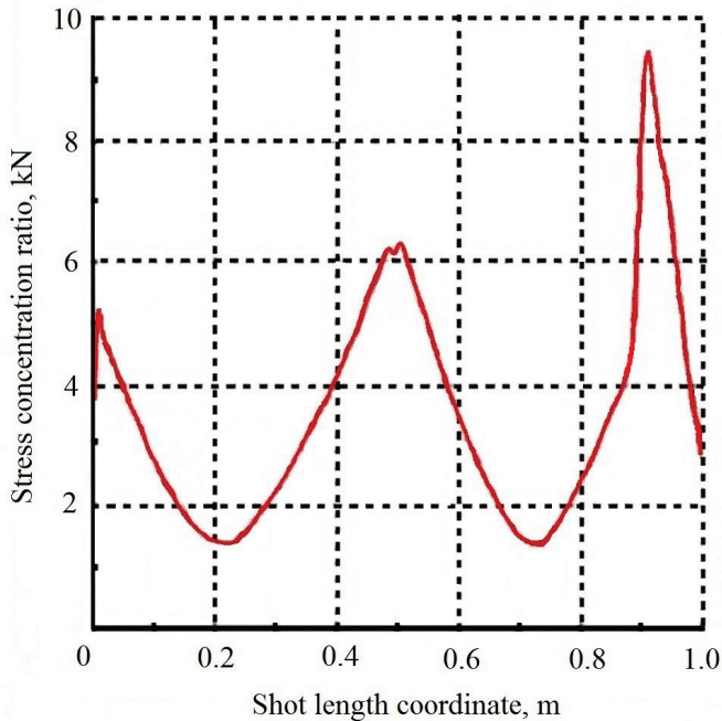
Fig. 12. Graph of distribution of stress concentration coefficient values along the length of a buntion with a defect.
