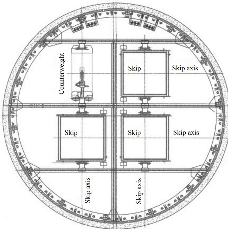
Fig. 2. Section skip shaft in the zone of movement of rocks.
