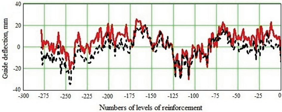
Fig. 5. Profiles of guides of an ore shaft in a zone of rock displacement of an ore-hoisting shaft in a frontal plane of guides.
