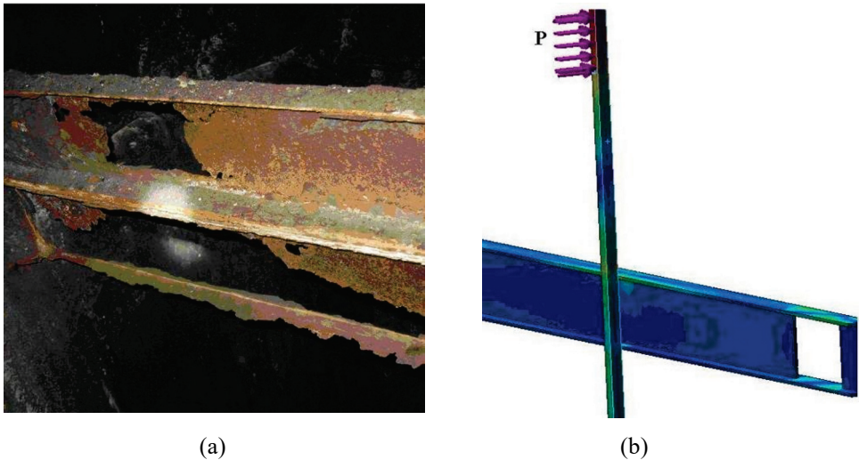
Fig. 6. Defects of buntions during long-term operation in aggressive mine environments: (a) – photographic materials; (b) – solid model of a guide-buntion system with a local defect.
