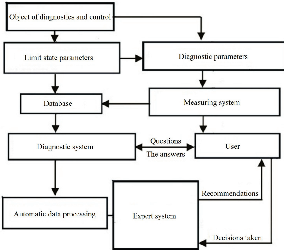
Fig. 14. Block diagram of the expert diagnostic system of mine hoists.
