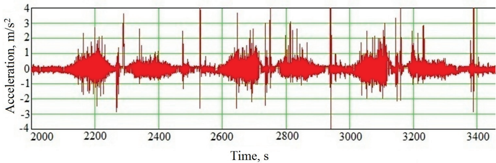
Fig. 10. Horizontal accelerations of vessel guides in lateral planes of reinforcement.
