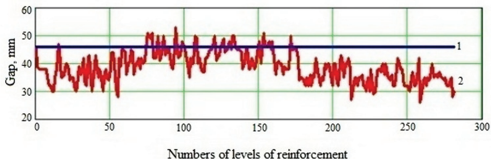
Fig. 8. Frontal gaps between conductors and sliding guides: 1 – maximum permissible level, mm; 2 – actual clearances, mm.
