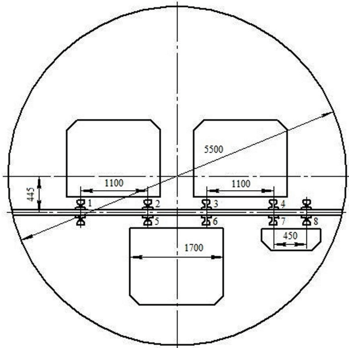
Fig. 1. The cross section of the coal barrel in the zone of displacement of rocks.
