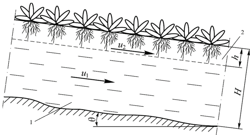
Fig. 2. Scheme of a non-pressure flow in a fluid channel with plants floating on a free surface [12]: 1 – non-pressure fluid flow, 2 – fluid flow in a porous layer; u_1, u_2 – velocity in layers, m/s; h – layer thickness with hyacinths, m; H – layer height from the bottom of the channel to the layer with hyacinths, m; \theta – channel bottom slope to the horizon, degrees.
