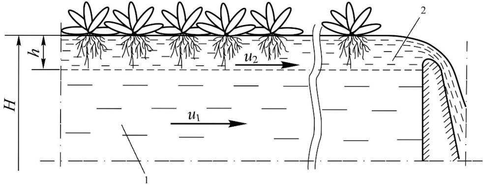
Fig. 3. Scheme of non-pressure fluid flow with plants floating on a free surface in clarifying-pond of the tailing pond [12]: 1 – non-pressure fluid flow, 2 – fluid flow in a porous layer.
