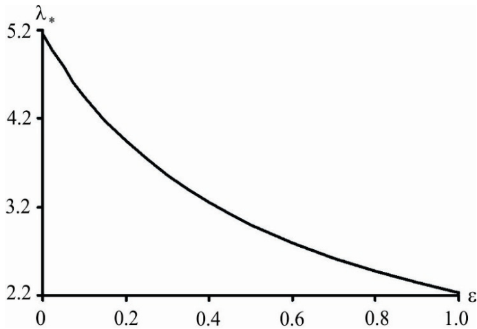
Fig. 5. The dependence of \lambda_* on the porosity of the layer from the plant on the surface.
