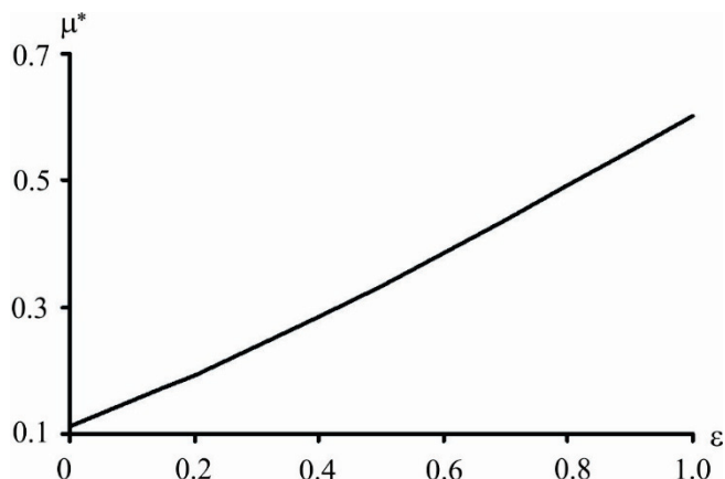
Fig. 6. The dependence of the maximum value of the velocity coefficient in the layer with plants floating on the free surface on the layer porosity.
