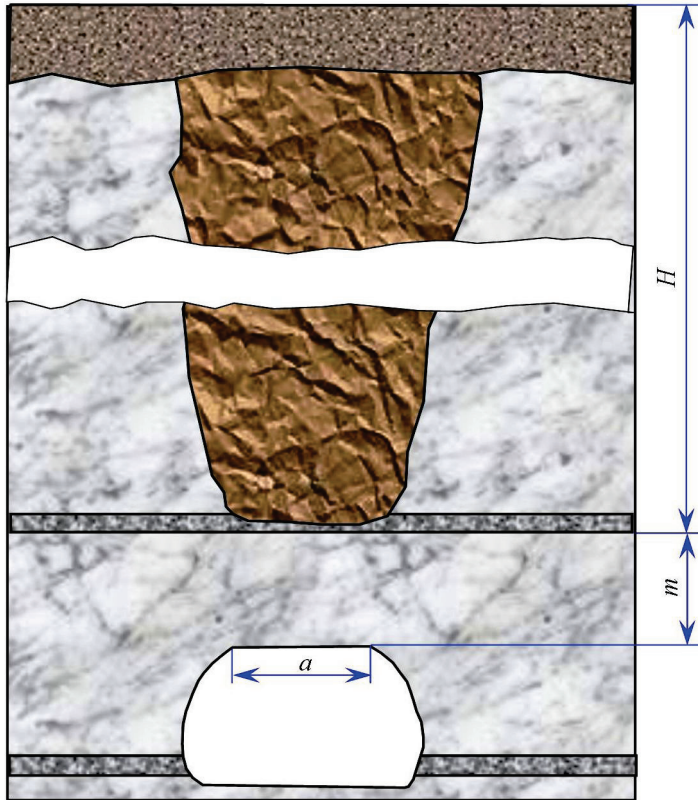
Fig. 4. To calculation of protective seam thickness in room roof for the most unfavorable scenario.
