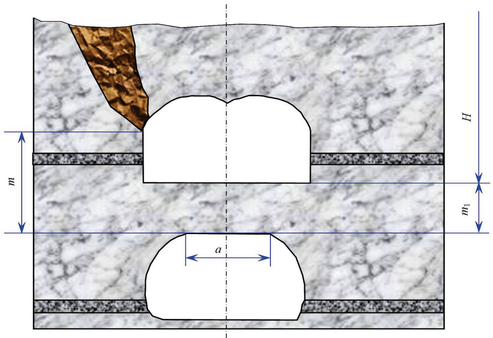
Fig. 6. Development of disturbed gypsum seam at two levels.
