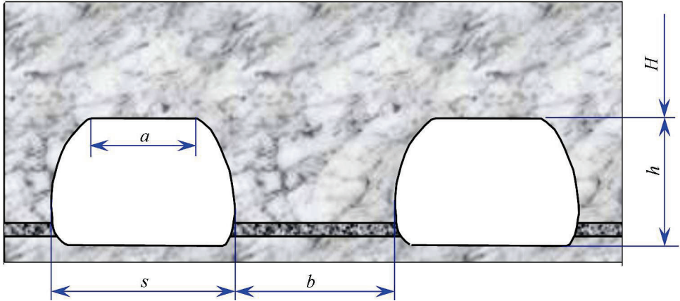
Fig. 8. To calculation of long safety pillar width.
