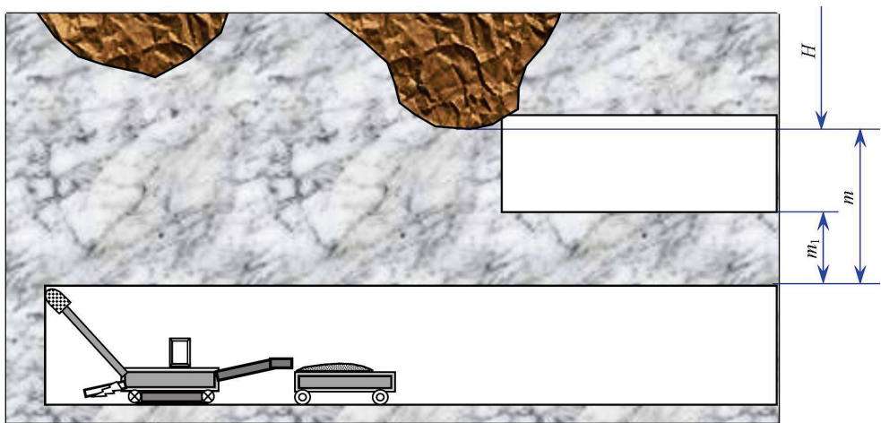
Fig. 7. Longitudinal cross-section for second development option.
