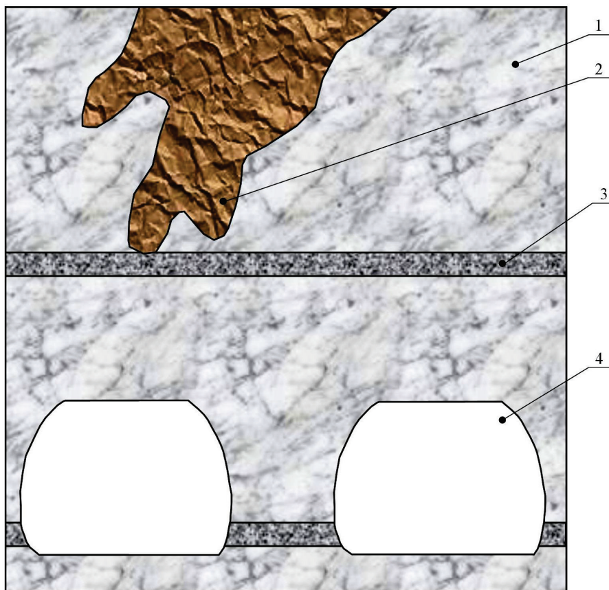
Fig. 3. Illustration of mining technology of disturbed gypsum seam: 1 – gypsum seam, 2 – karst, 3 – layer of dolomite, 4 – mine working.
