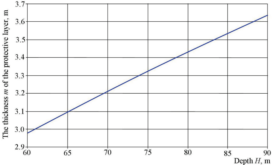
Fig. 5. Dependency between protective seam thickness of room roof on mark depth of room roof with a karst above the middle dolomite.
