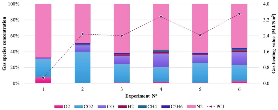
Fig. 7. Low heating value of the syngas as a function of gas species concentration
