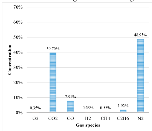
Fig. 2. Syngas composition – Experiment no. 2
