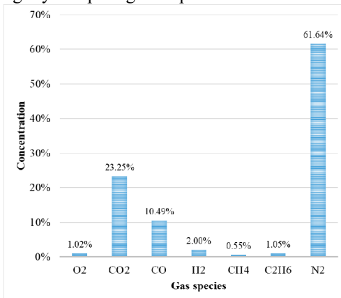
Fig. 3. Syngas composition – Experiment no. 3
