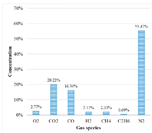
Fig. 6. Syngas composition – Experiment no. 6
