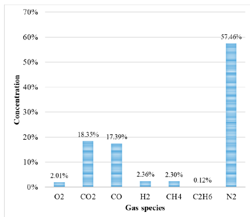
Fig. 4. Syngas composition – Experiment no. 4
