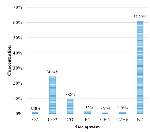
Fig. 5. Syngas composition – Experiment no. 5
