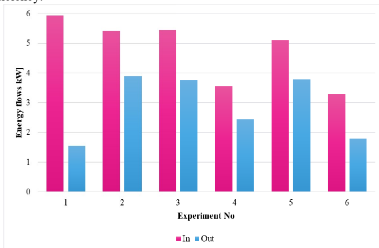
Fig. 10. Energy balance of the gasification experiments
