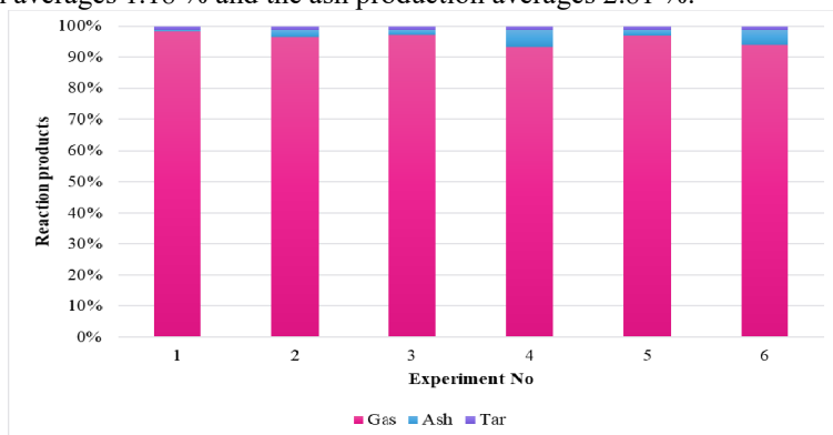
Fig. 9. Reaction products distribution of the gasification experiments
