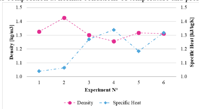
Fig. 8. Density and specific heat of the syngas
