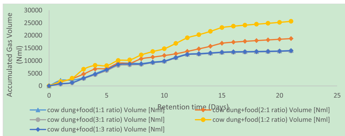
Fig. 4. Accumulated gas volume with time
