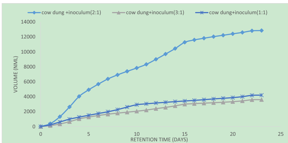
Fig. 6. Accumulated gas volume for mono-digested cow dung
