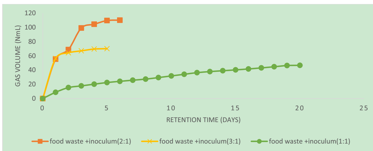
Fig. 5. Accumulated gas volume for mono-digested food waste
