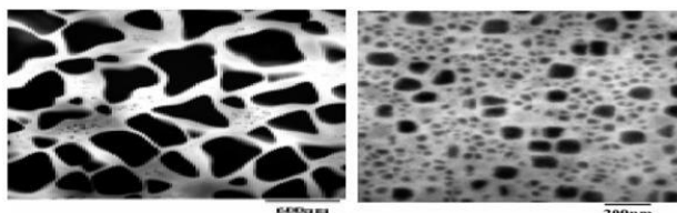
Fig 7: Secondary and Tertiary \gamma' phases in nickel based super alloys [5]
