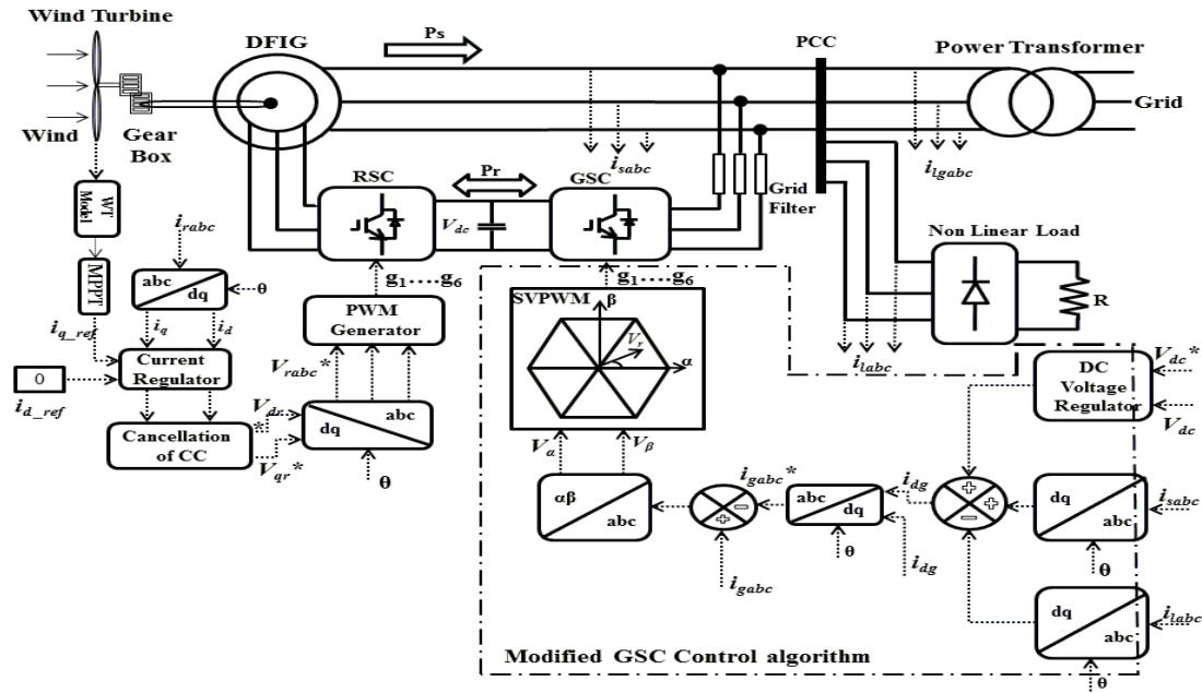
Fig. 2. Proposed SVPWM based Modified GSC control technique for DFIG based WECS.
