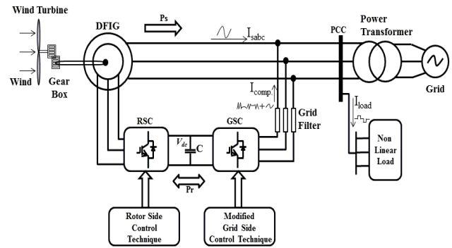
Fig. 1. Basic block diagram of grid-connected DFIG based WECS system
