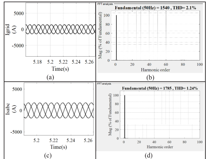
Fig. 7. DFIG performance under nonlinear load condition (a) I_{grid} (grid current), (b) %THD of I_{grid} , (c) I_{sabc} (Stator current), (d) %THD of I_{sabc} .
