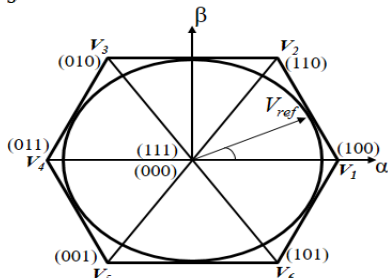
Fig. 4. The hexagonal structure of the SVPWM technique.
