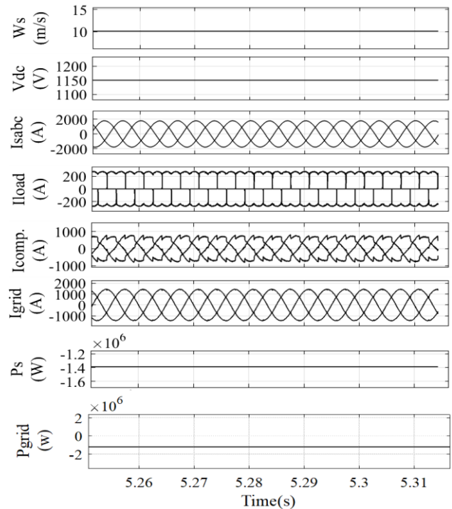
Fig. 6. DFIG performance with the proposed modified GSC control technique under 10.09 m/s wind speed.
