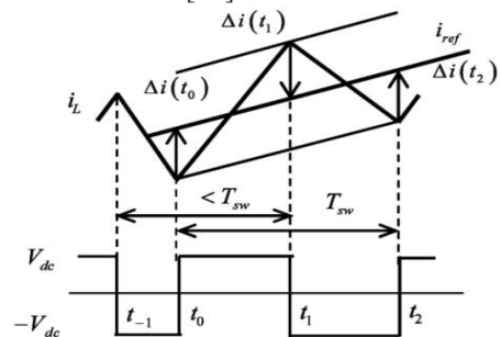
Fig. 3. Hysteresis current control PWM controller
