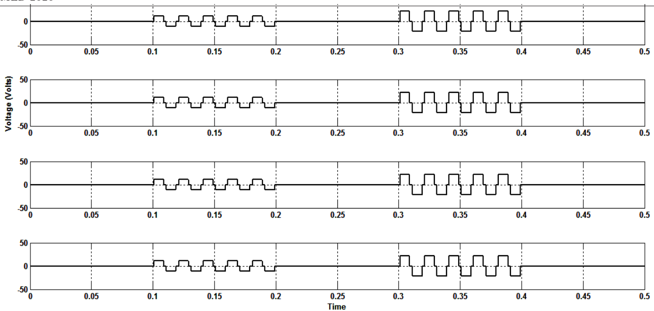
Fig. 8. Injected voltage waveforms.
