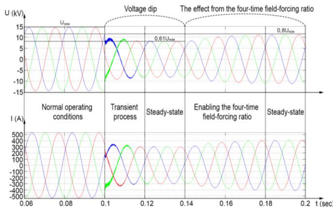
Fig. 7. Oscillogram of phase voltages and SEM currents at the time four-time field forcing.
