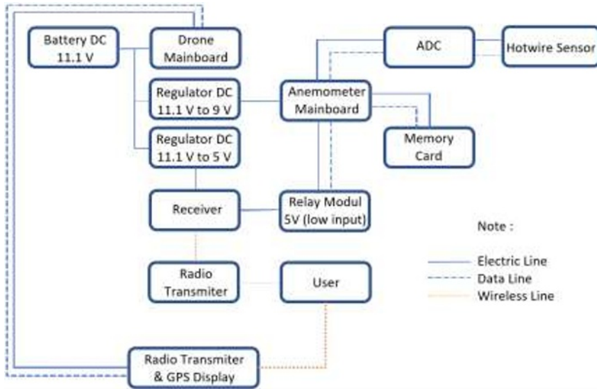
Fig. 4. Flow diagram of anemometer surveyor drone.
