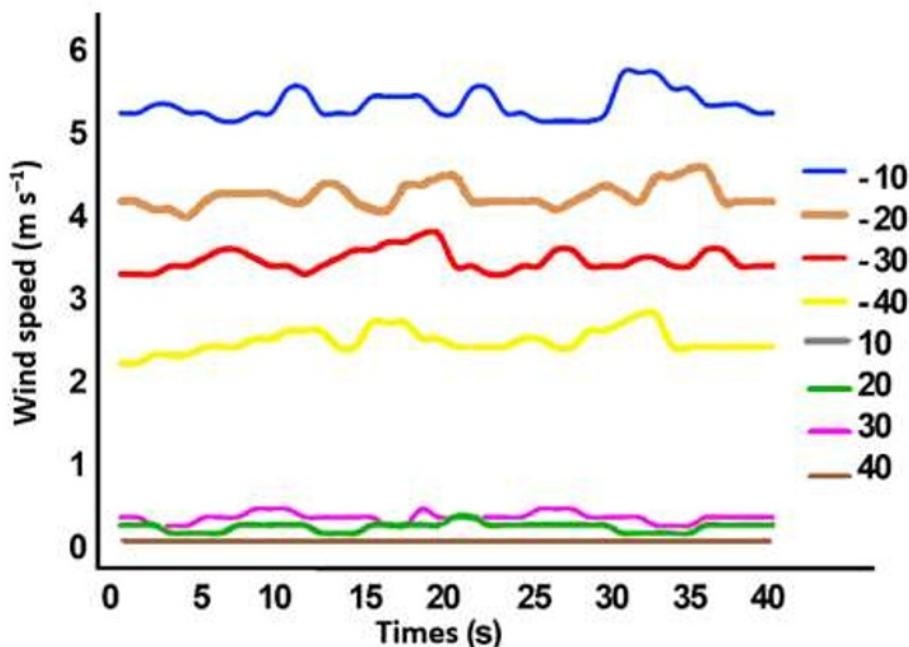
Fig. 1. Graph of wind velocity.
