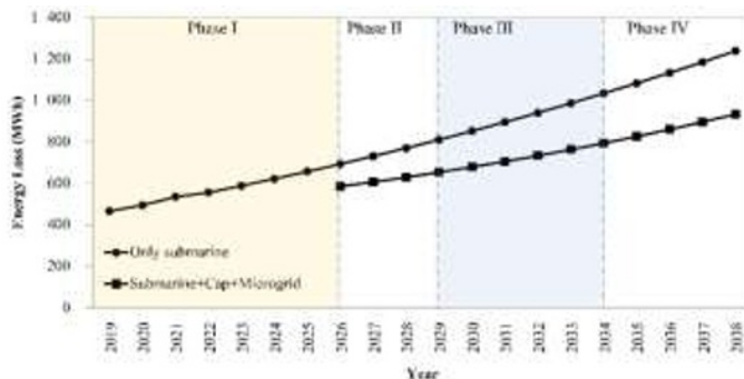
Fig. 10. Simulation results of energy loss in the feeder No.10, comparing between (i) only submarine cable, and (ii) submarine cable, capacitor bank and microgrid installation.
