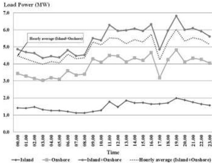
Fig. 4. Load profiles of peak demand occurring on April 13, 2018 and hourly average of load profile in 2018 at Sichang island and onshore [16].
