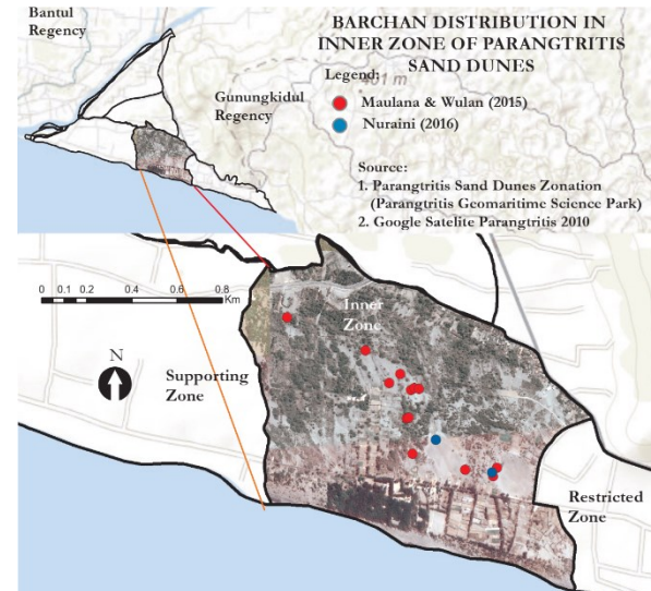
Fig. 2. Barchan dunes distribution in Inner Zone of Parangtritis coast. Barchan dune identified using UAV by Maulana & Wulan in 2015 (red dots). Barchan dune identified during a field survey by Nuraini in 2016 (blue dots).
