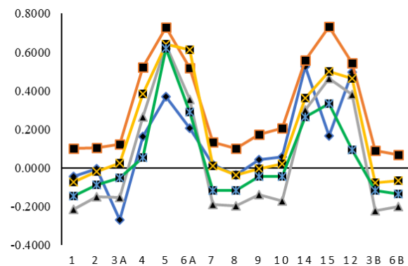
Fig. 5. NDVI value on each barchan in 2015 (blue line), 2016 (orange line), 2017 (grey line), 2018 (yellow line), & 2019 (green line).
