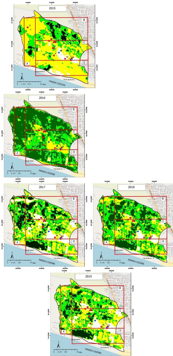
Fig. 4. The vegetation covers changed in Inner Zone. White areas illustrate no vegetation cover, yellow areas slightly density, green areas moderately density, and dark green areas high density.
