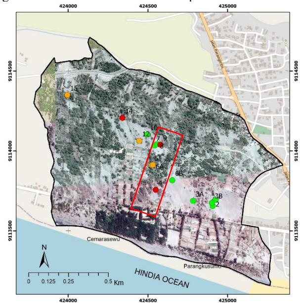
Fig. 7. Slip face height changes in the Inner Zone of the Parangtritis coastal area. Green dots represent barchan with no changes, while orange dots for barchan with slightly changed, and red dots for barchan with changed class.
