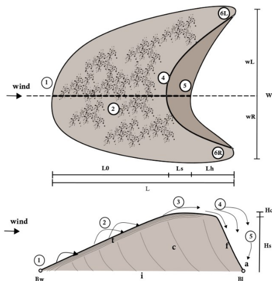
Fig. 1. Barchan dune morphology, morphometry, & structures. Morphology: (1) windward toe, (2) windward side, (3) crest, (4) brink, (5) slip face, (6) horns (L= left, R= right). Morphometric: L , length of barchan; L_0 , length from toe to the brink; L_s , length of slip face; L_h , length of horn; W , the width of barchan; w_L , the width of the left horn; w_R , the width of the right horn; H_c , the height of barchan; H_s , the height of the slip face; B_w , windward bottom; B_l , lee bottom. Structure: t , top set; c , tabular-planar cross bed set; f , foreset; a , apron deposits; i , interdune deposits. (Modified from [6])
