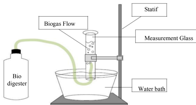
Fig 1. Schematic diagram of bioreactor in laboratory scale
