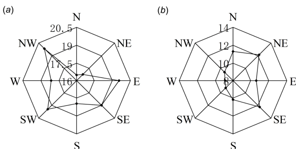
Fig. 4. RMSE changes with aspects for GDEM minus DGPS (a), SRTM3 minus DGPS (b)
