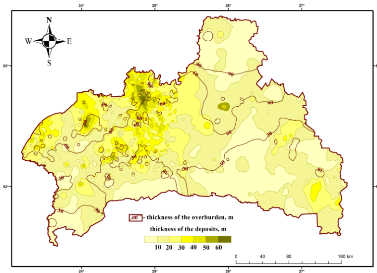
Fig. 8. Thickness of the Neogene sediments of the Brest region
