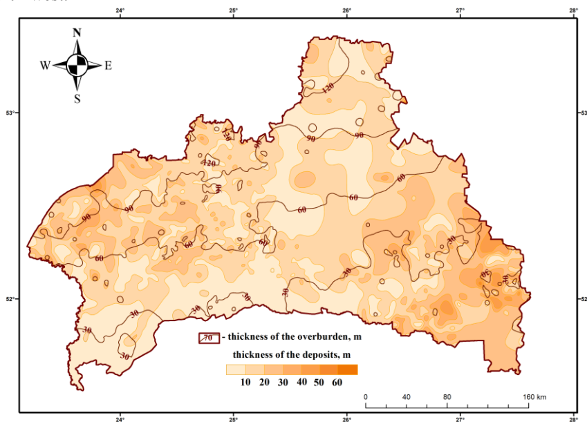
Fig. 6. Thickness of Paleogene sediments of the Brest region
