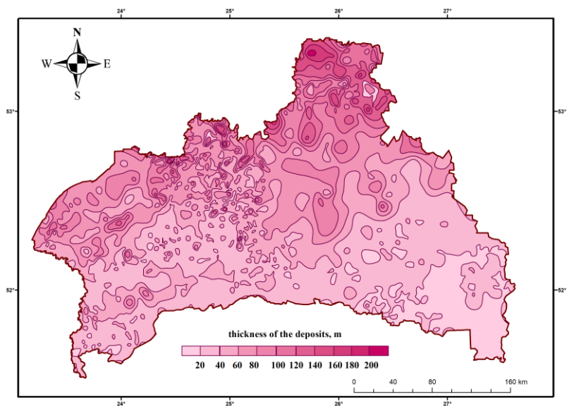
Fig. 10. The thickness of the Quaternary sediments of the Brest region
