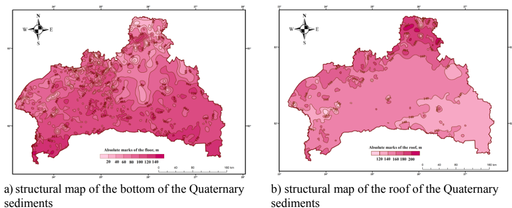
Fig. 9. Structural maps made for the Quaternary sediments of the Brest region
