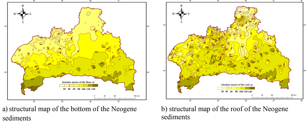
Fig. 7. Structural maps made for the Neogene sediments of the Brest region
