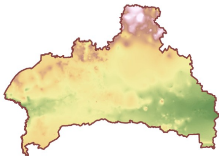
c) an example of using the natural neighborhood method
