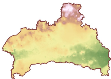
a) an example of using the inverse distance weighted method
