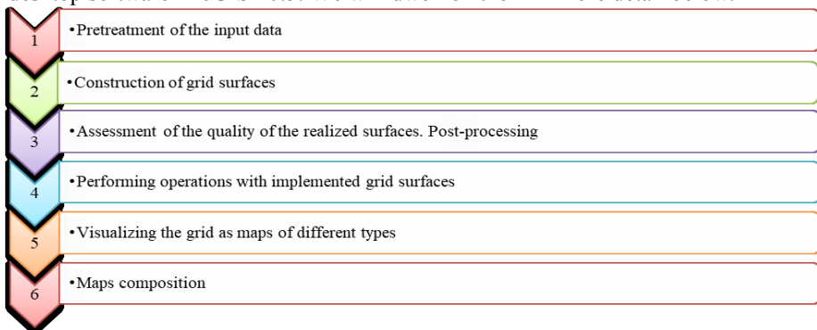
Fig. 2. The method of creating a set of structural geological maps of the Cenozoic deposits of the Brest region
