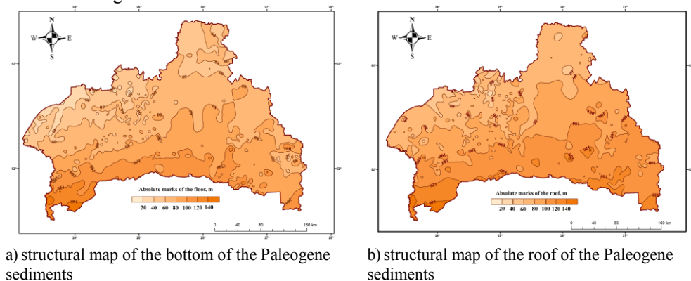
Fig. 5. Structural maps made for the Paleogene sediments of the Brest region
