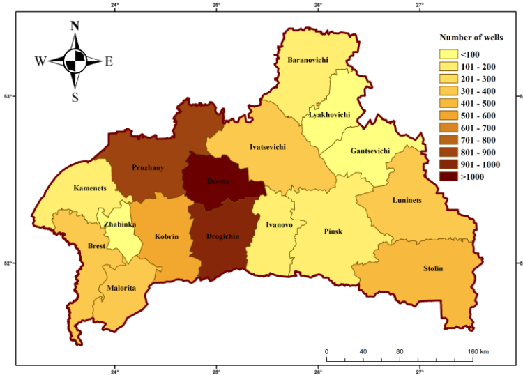
Fig. 1. Information on the number of boreholes in the context of the administrative districts of the Brest region
