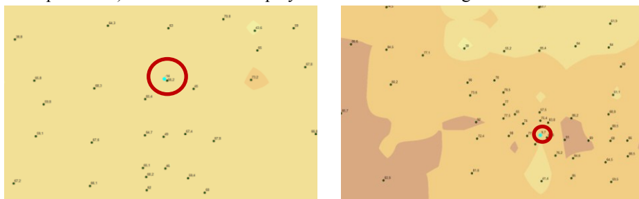
Fig. 3. Data errors identified using the kriging tool
